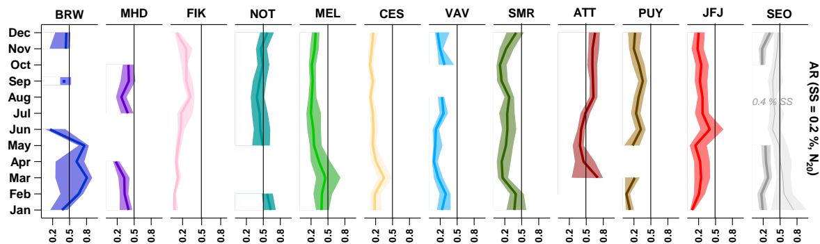
Fig. S5: Annual cycle of the CCN activation ratio at SS = 0.2 %. The basis for the total particle number is N_{20} . The thick colored lines indicate the median activation ratio, while the shaded colored areas show the interquartile range. The black vertical bars indicate 50 % activation. Due to higher data coverage in SEO results for SS = 0.4 % are shown additionally.
