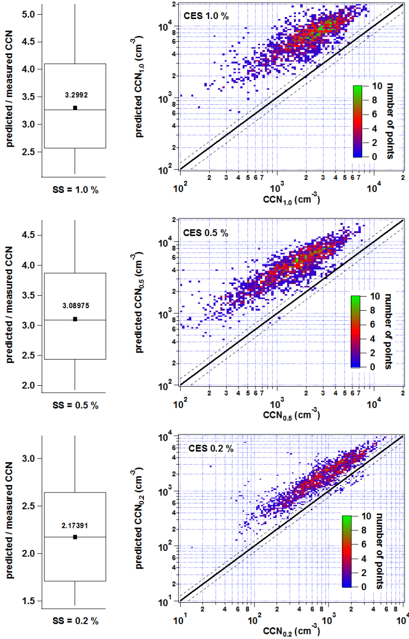
Fig. S2: Performance of closure study for the CES data set at SS = 1.0, 0.5 and 0.2 %. The left panels show the ratio of the predicted CCN number concentration based on the \kappa -Köhler theory and the measured CCN number concentration as a box and whiskers plot. The box indicates the interquartile range, the whiskers the 10 th and 90 th percentiles, the middle horizontal bar the median and the marker the geometric mean whose value is also given. The right panels show the relationship between the predicted and measured CCN number concentrations within logarithmic bins. The color code indicates the number of particles falling within one bin space. The solid black line is the 1:1 line while the dashed lines mark the 10 % particle uncertainty range.
