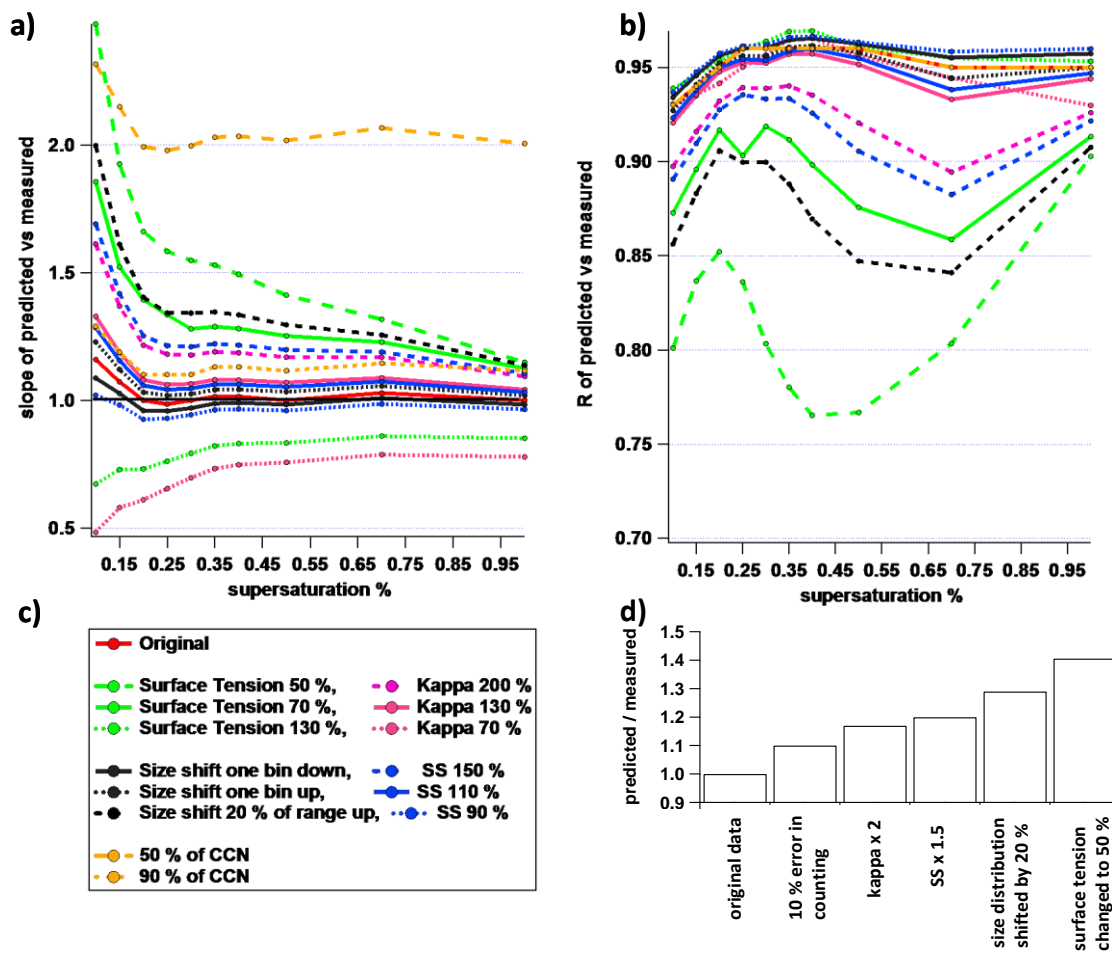
Fig. S3: Sensitivity analysis of a \kappa -Köhler closure study based on the uncorrected JFJ data. Panel (a) shows how the agreement between the predicted and measured CCN number concentration changes with supersaturation in form of the slope of the linear regression. Panel (b) shows the same for the correlation coefficient. The legend is given in panel (c), while (d) summarizes the top panels by showing how the prediction skill changes when varying specific variables by extreme values.
