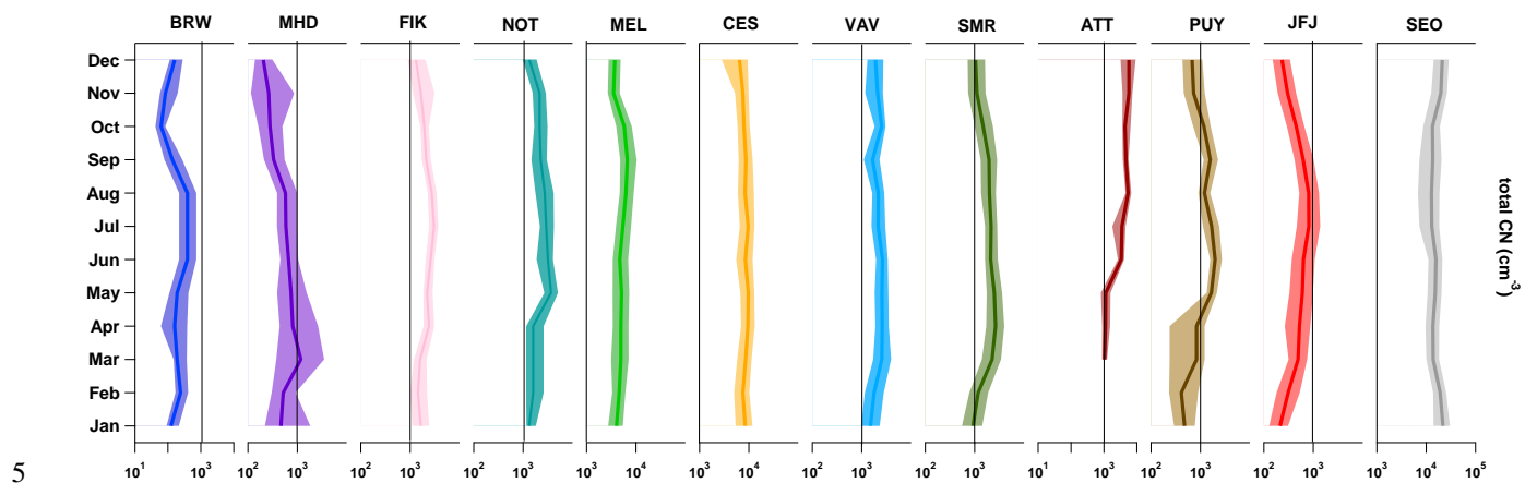
Fig. S4: Seasonal cycle of the total number concentration. The thick colored lines indicate the median value, while the shaded colored areas show the interquartile range. The black vertical bars indicate 1000 particles \text{cm}^{-3} .
