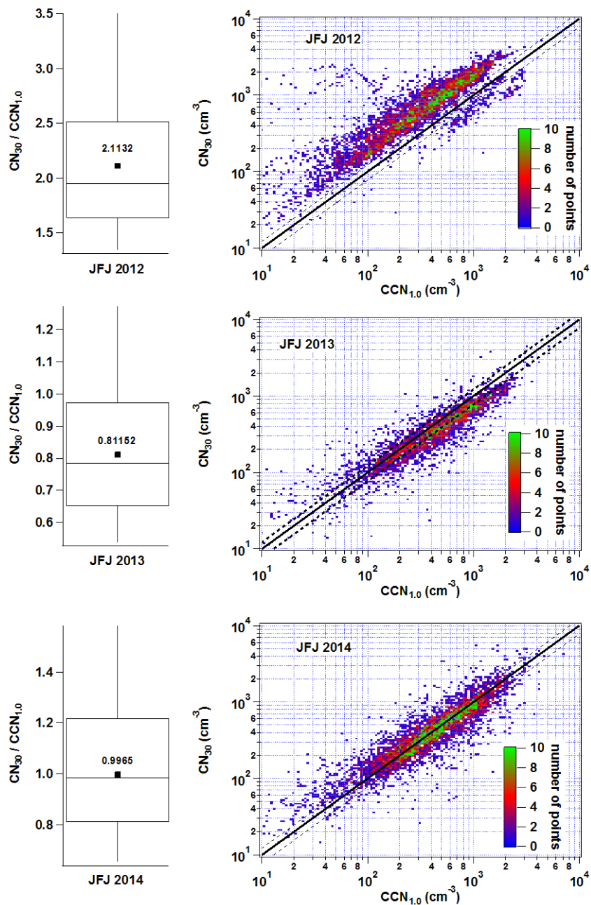
Fig. S1: Untreated JFJ data from 2012, 2013 and 2014. The left panels show the ratio of the total particle number > 30 nm and the CCN number concentration at SS = 1.0 % as a box and whiskers plot. The box indicates the interquartile range, the whiskers the 10 th and 90 th percentiles, the middle horizontal bar the median and the marker the geometric mean whose value is also given. The right panels show the relationship between CN_{30} and CCN_{1,0} within logarithmic bins. The color code indicates the number of particles falling within one bin space. The solid black line is the 1:1 line while the dashed lines mark the 10 % particle uncertainty range.
