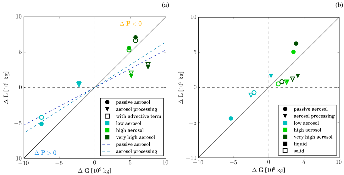
Figure 8. (a) Scatterplot of change in condensate gain \Delta G and loss \Delta L relative to the simulation with the standard aerosol profile. Points falling above the one-to-one line (solid black line) portray a decrease in surface precipitation, while points below it portray a surface precipitation increase. For points in the area between the solid black line and the dashed lines (dark blue: passive aerosol, light blue: aerosol processing) the change in condensate generation dominates over the change in precipitation efficiency (Appendix B). The impact of advection of condensed water out of the domain is illustrated by the open symbols. For these points the advective flux is discounted as loss. (b) Same as (a), but separating contribution of condensation and evaporation (filled symbols) from contribution of deposition and sublimation (open symbols).
