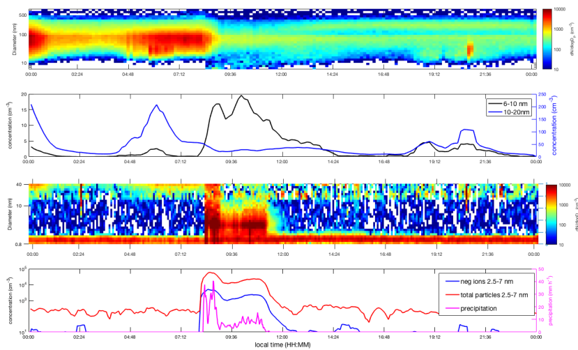
Fig. 2. Figure 7. Example for a rain-induced event for total particles (DMPS). The DMPS measurements are taken above the canopy (60 m height), NAIS measurements are inside the canopy. Panel (a) shows the DMPS
