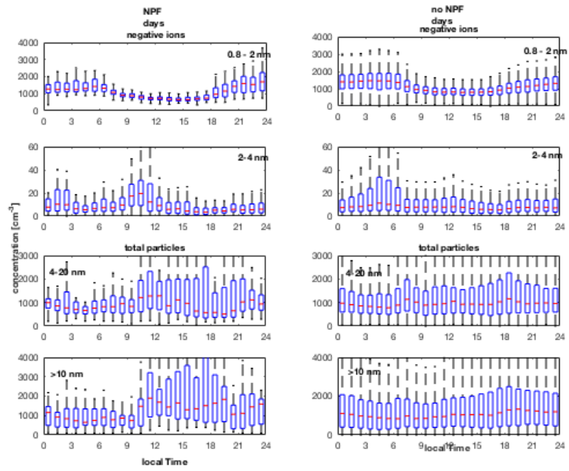
Fig. 3. Figure 9. Diel cycle of ions measured outside the canopy by the NAIS (small: 0.8–2 nm; intermediate: 2–4 nm; The lowest two panels show the total particles (large: 4–20 nm) from the NAIS and total par
