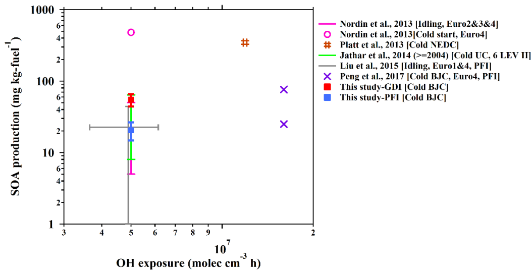
556 Figure 5. Fuel-based SOA production from gasoline vehicle exhaust as a function of OH exposure in the chamber 557 simulations. The SOA production data are from published studies of chamber simulation of gasoline vehicle 558 exhaust. From the study of Jathar et al. (2014), the SOA production of vehicles manufactured in 2004 or later (LEV 559 II) is selected, which is a model year that is more close to those of the vehicles in this study. The error bars of 560 previous results indicate the range of OH exposure (x axis) and SOA production (y axis) in their simulations. The 561 driving cycles and vehicle information are also noted in the legend of each study.
