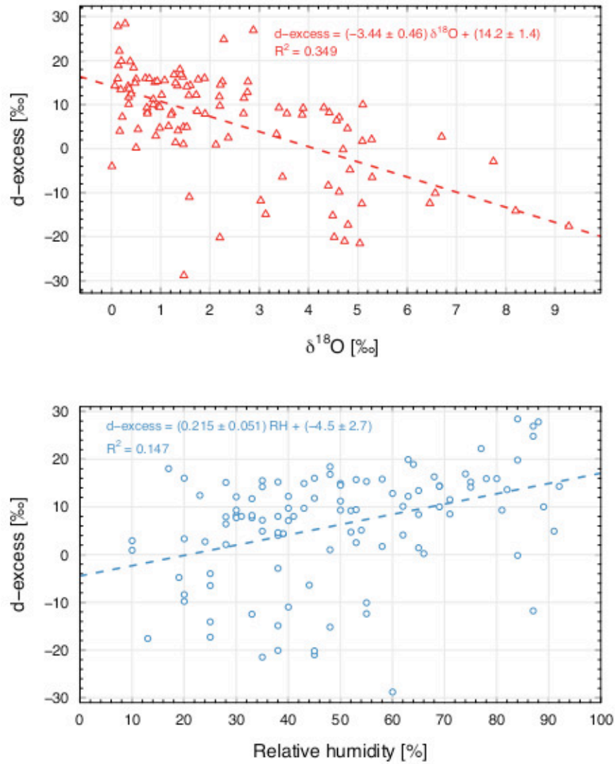
Figure 8. Upper diagram: relationship between deuterium excess and positive \delta^{18}\text{O} values measured in daily precipitation samples collected by six stations distributed along southern foothills of the Himalayas (cf. Fig. 1). Lower diagram: relationship between deuterium excess and relative humidity of the local, near-ground atmosphere (daily means) calculated for precipitation events exhibiting positive \delta^{18}\text{O} values.
