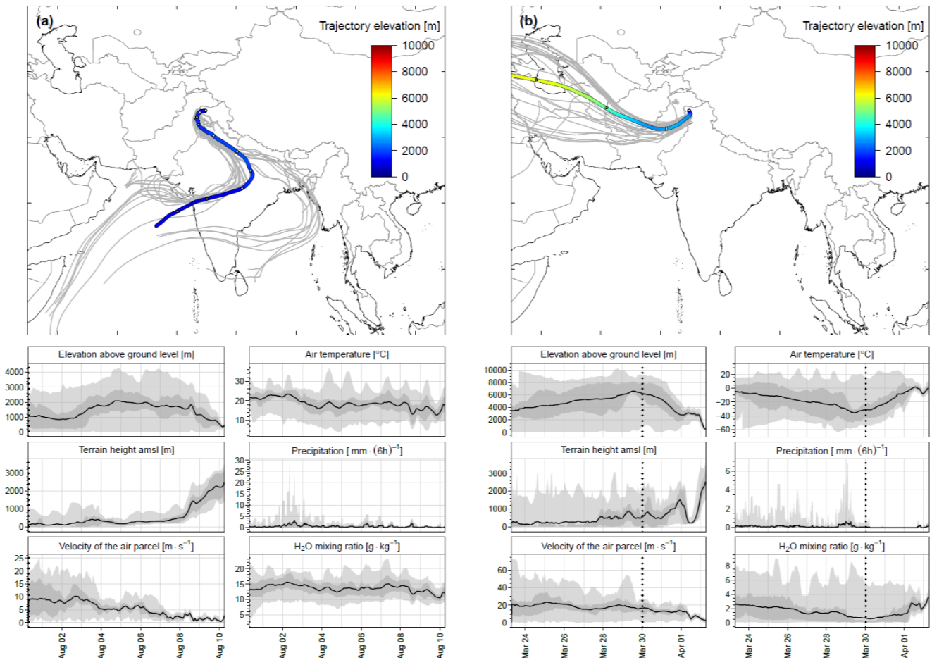
5 Figure 7. (a) upper diagram: 10-day backward trajectories arriving at Srinagar station on August 10, 2010, 12:00 hours and representing Indian Summer Monsoon (ISM) period. (b) Upper diagram: 10-day backward trajectories arriving at Srinagar station on April 2, 2011, 12:00 hours and representing Western Disturbances (WD) period. Twenty seven ensembles (grey lines in the background) and the mean trajectory (heavy line) are shown. Colours of the mean trajectory indicate elevation above the local ground in meters. Empty white dots on the mean trajectory indicate 24-hour intervals. Lower diagrams of (a) and (b) show the evolution of six selected parameters of air parcel along the trajectory. Evolution of the mean value of each parameter is marked by heavy black line and the associated uncertainty in grey. Dashed vertical lines mark part of the mean 10 10-day trajectory visible in the upper diagram. International boundaries are only indicative and as provided by the software.
