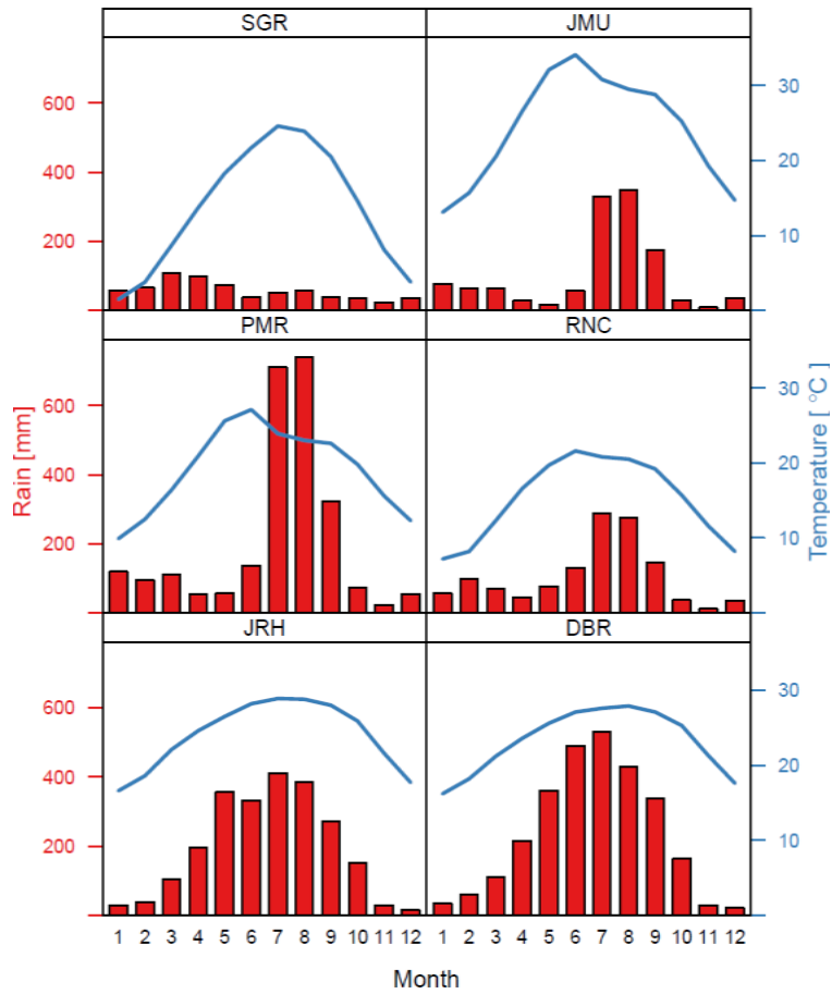
Figure 2. Long-term (1985-2014) monthly surface air temperature and precipitation data for six stations where daily sampling of rainfall for isotope analyses was conducted. SGR - Srinagar, JMU - Jammu, PMR - Palampur, RNC - Ranichauri, JRH - Jorhat, DBR - Dibrugarh. Source of data: Srinagar, Jammu, Palampur, Jorhat, Dibrugarh - pl.climate-data.org ; Ranichauri - Upadhyay et al., 2015.
