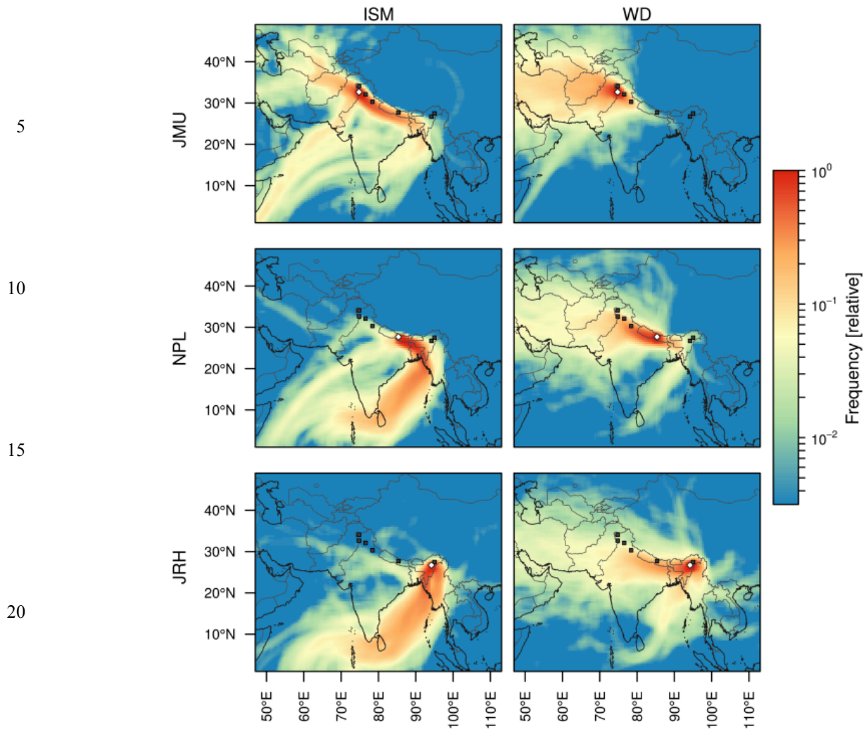
25 Figure 9. Footprint maps of air masses arriving at three stations: Jammu (JMU), Kathmandu (NPL) and Jorhat (JRH) 30 representing western, central and eastern part of the studied east-west transect along southern foothills of the Himalayas , respectively (top, middle and bottom graphs). Separate maps were prepared for Indian Summer Monsoon (ISM) and Western Disturbances (WD) periods. Daily trajectories for the period 2009-2011 were reconstructed using Hysplit modelling framework (see text for details). International boundaries are only indicative and as provided by the software. Colour scale indicates the focally averaged number of trajectories passing through a grid cell.
