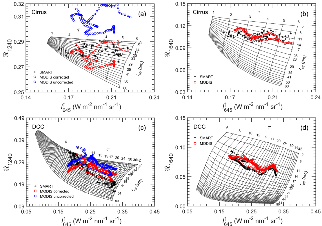
Figure 8. Radiance lookup tables for the cirrus case (a,b) and DCC case (c,d). (a) and (c) are using C1 ( I_{645}^\uparrow and \mathfrak{R}_{1240} ), while (b) and (d) are using C2 ( I_{645}^\uparrow and \mathfrak{R}_{1640} ). For the cirrus case, the simulations are performed with \theta_0 = 37^\circ and assuming GHM (Baum et al., 2014), while for the DCC case \theta_0 = 26^\circ and the ice habit of plate (Yang et al., 2013) are applied. Radiance measurements of SMART and MODIS are illustrated by symbols.
