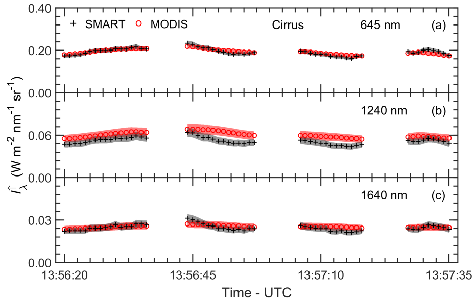
Figure 4. Time series of I_{\lambda}^{\uparrow} centered at \lambda = 645 \text{ nm} (a), 1240 \text{ nm} (b), and 1640 \text{ nm} (c) measured by SMART (black) and MODIS (red) for the cirrus case. Shaded areas are measurement uncertainties. Gaps on the time series indicate when the shutter of SMART closed for dark current measurements.
