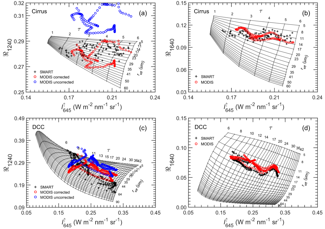
Figure 8. Radiance lookup tables for the cirrus case (a,b) and DCC case (c,d). (a) and (c) are using C1 ( I_{645}^{\uparrow} and R_{1240} ), while (b) and (d) are using C2 ( I_{645}^{\uparrow} and R_{1640} ). For the cirrus case, the simulations are performed with \theta_0 = 37^\circ and assuming GHM (Baum et al., 2014), while for the DCC case \theta_0 = 26^\circ and the ice habit of plate (Yang et al., 2013) are applied. Radiance measurements of SMART and MODIS are illustrated by symbols.
