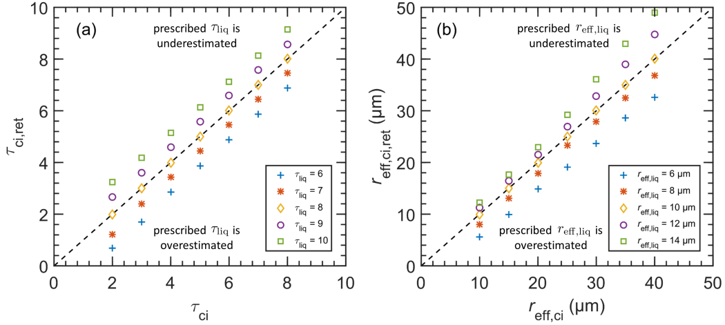
Figure 9. Comparison of synthetically retrieved \tau_{\text{ci}} (a) and r_{\text{eff},\text{ci}} (b). Calculations in (a) are performed by changing \tau_{\text{liq}} while the original value is 8 and r_{\text{eff},\text{ci}} = 20 \mu\text{m} and r_{\text{eff},\text{liq}} = 10 \mu\text{m} are fixed. In (b), r_{\text{eff},\text{liq}} is changed while the original value is 10 \mu\text{m} and \tau_{\text{ci}} = 3 and \tau_{\text{liq}} = 8 are fixed.
