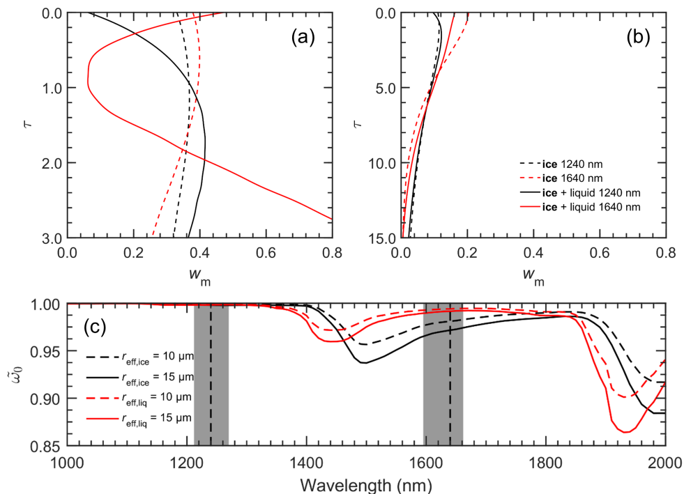
Figure 12. (a) is w_m at \lambda = 1240 \text{ nm} and 1640 \text{ nm} calculated for cloud A, while (b) is for cloud B. Solid line and dashed line describe w_m calculated with and without the presence of underlying liquid water cloud, respectively. (c) Single scattering albedo \tilde{\omega}_0 of GHM and liquid water droplets with r_{\text{eff}} of 10 \mu\text{m} and 15 \mu\text{m} .
