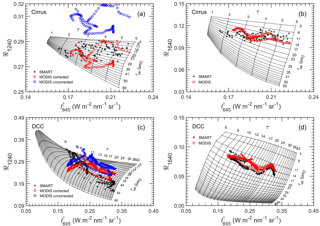
Figure 8. Radiance lookup tables for the cirrus case (a,b) and DCC case (c,d). (a) and (c) are using C1 ( I_{645}^{\uparrow} and \Re_{1240} ), while (b) and (d) are using C2 ( I_{645}^{\uparrow} and \Re_{1640} ). For the cirrus case, the simulations are performed with \theta_0 = 37^\circ and assuming GHM (Baum et al., 2014), while for the DCC case \theta_0 = 26^\circ and the ice habit of plate (Yang et al., 2013) are applied. Radiance measurements of SMART and MODIS are illustrated by symbols.
