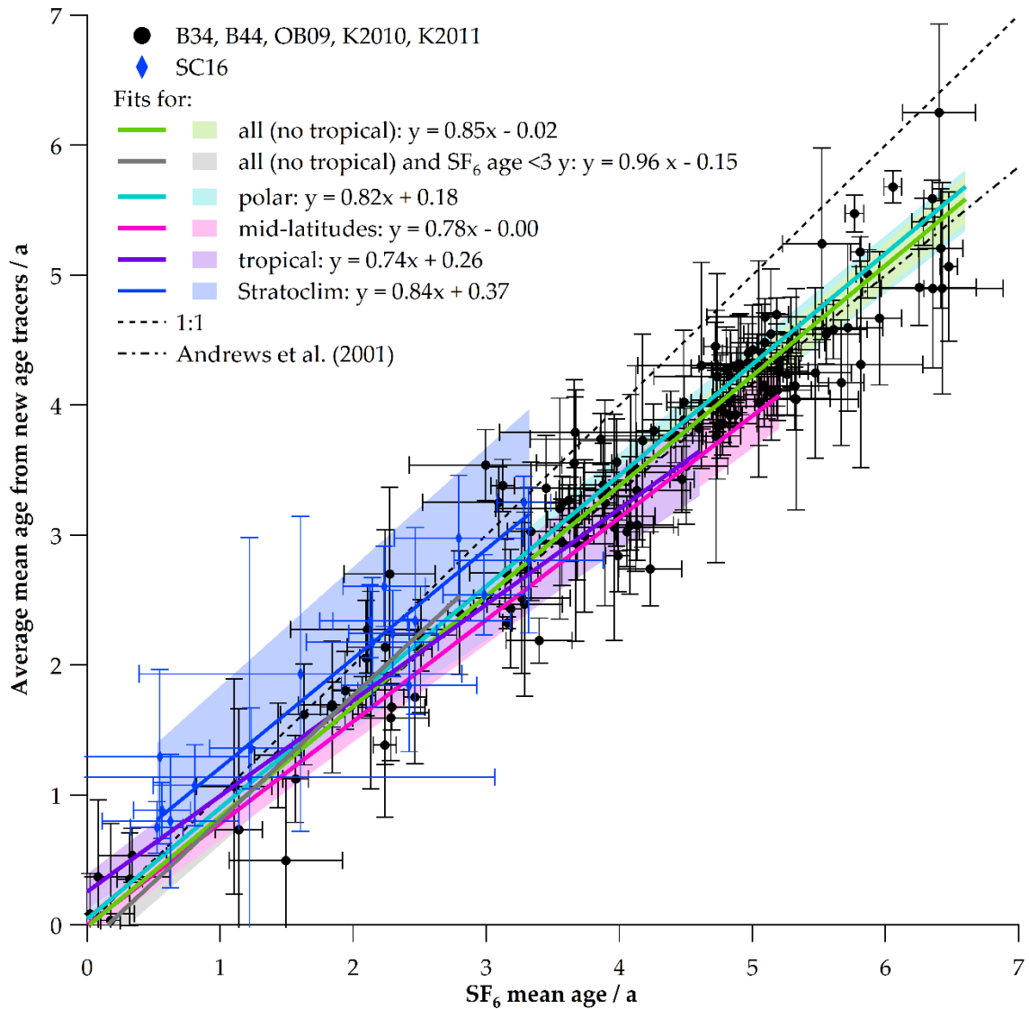
Figure 4. ‘Best estimate’ mean ages (a combined mean age based on CF 4 , C 2 F 6 , C 3 F 8 , CHF 3 and HFC-125) plotted against SF 6 mean age. Error bars are based on stratospheric uncertainties from Table 3 column b. All fits are bivariate linear fits with uncertainties shown by shaded areas (see inset legend). SF 6 vs CO 2 line from Andrews et al. (2001) included for comparison.
