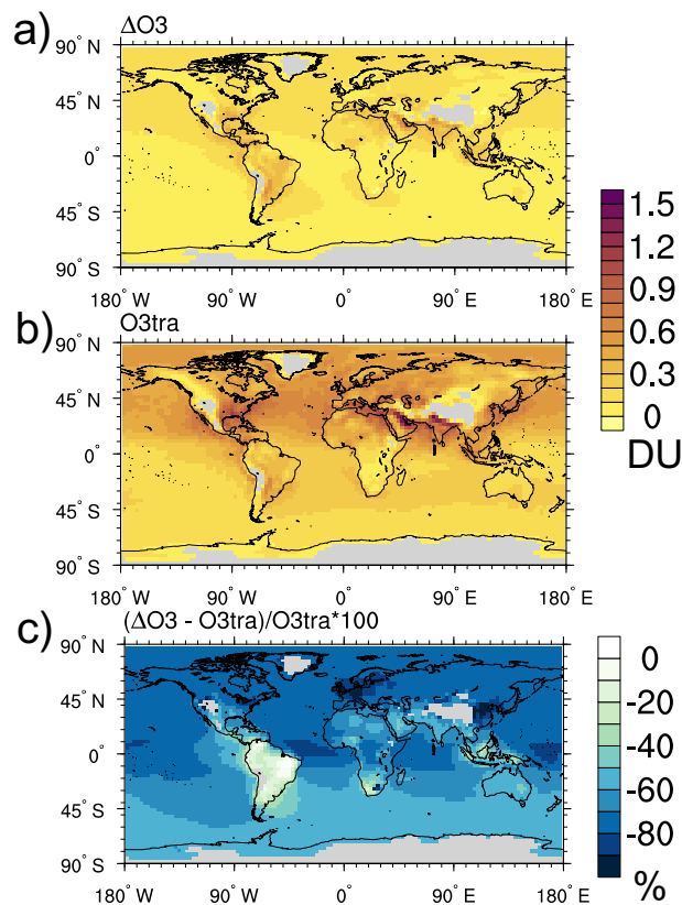
Figure 4. Multi-annual averages (2006–2010) of (a) \Delta O_3 (impact), (b) O_3^{\text{tra}} (contribution, both in DU) of the REF simulation and (c) the relative difference between the impact and the contribution of land transport emissions (in %). All values are calculated for the partial columns from the surface of up to 850 hPa (850PC).
