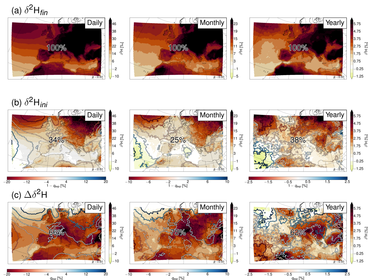
Figure 10. Difference in \delta^2\text{H} between the high and low anomaly days (left), months (middle), and years (right) at each grid point. The top row shows the mean \delta^2\text{H} in water vapour averaged over the first, third and fifth lowest model level, the middle and bottom rows show the weighted contributions of the initial values and the changes along the trajectories, respectively. The numbers show the mean contribution of each term to \delta^2\text{H}_{fin} , and the contours show the difference in 1 - q_{exp} (middle) and q_{exp} (bottom) in %. Stippling indicates areas where p < 0.01 . Note the different colour scales.
