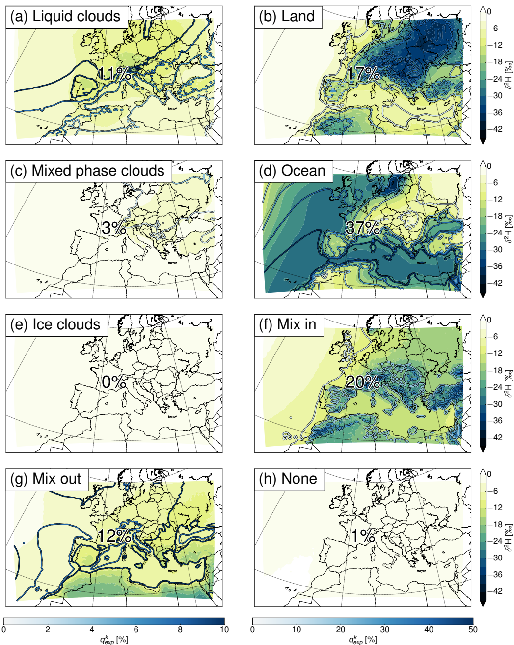
Figure 8. Contributions of the processes to \Delta\delta^2\text{H} in Figure 7 e. The numbers show the mean contribution of each process and the contours show q_{exp}^k (see Equations 10 and 11) in %. Note the different colour scales for q_{exp}^k between the left and right hand side.
