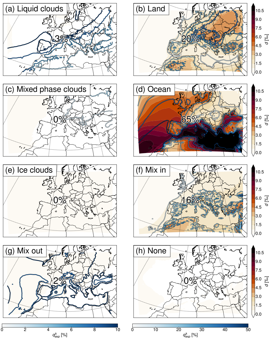
Figure 9. Contributions of the processes to \Delta d in Figure 7f. The numbers show the mean contribution of each process and the contours show q_{exp}^k (see Equations 10 and 11) in %. Note the different colour scales for q_{exp}^k between the left and right hand side.
