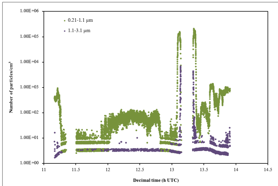
45 Figure A. Aerosol total number concentrations measured by the PCASP instrument for the 0.21-1.1 \mu\text{m} size range (green dots) and for the 1.1-3.1 \mu\text{m} size range (purple dots).
