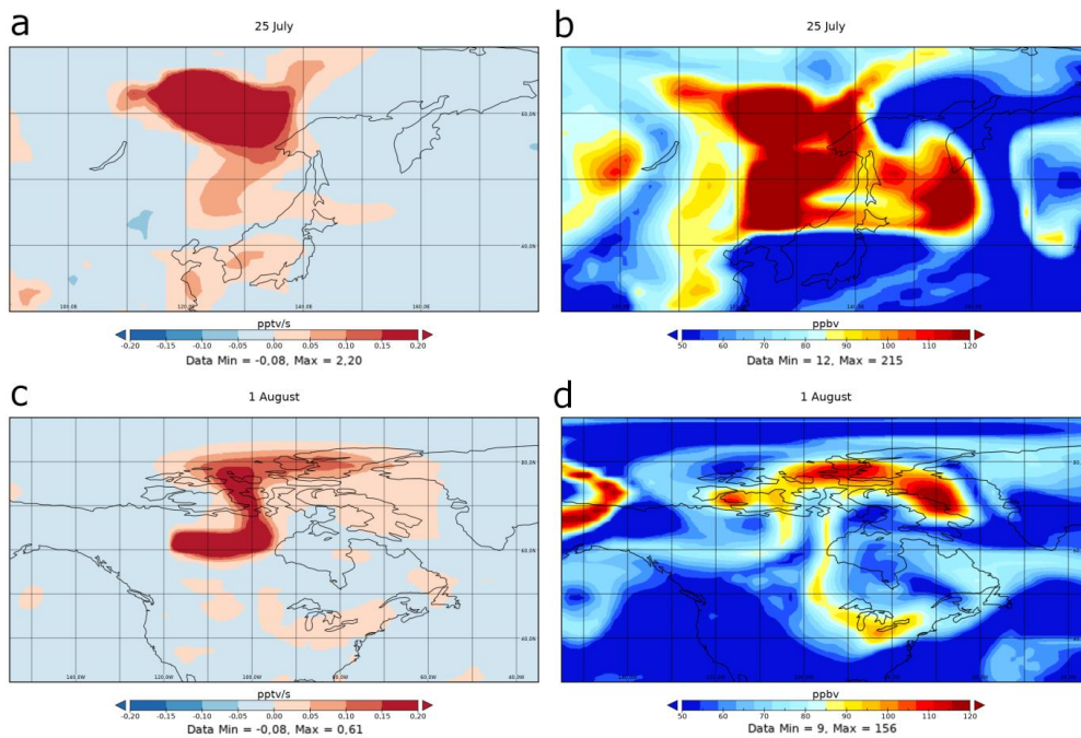
Figure 9. (a and c) Production of \text{O}_3 (in \text{pptv s}^{-1} ) and (b and d) concentrations of \text{O}_3 (in ppbv) on 25 July over Siberia (upper panels) and 1 August 2014 over North America (lower panels) at 5.5 km in altitude simulated by the MOCAGE model.
