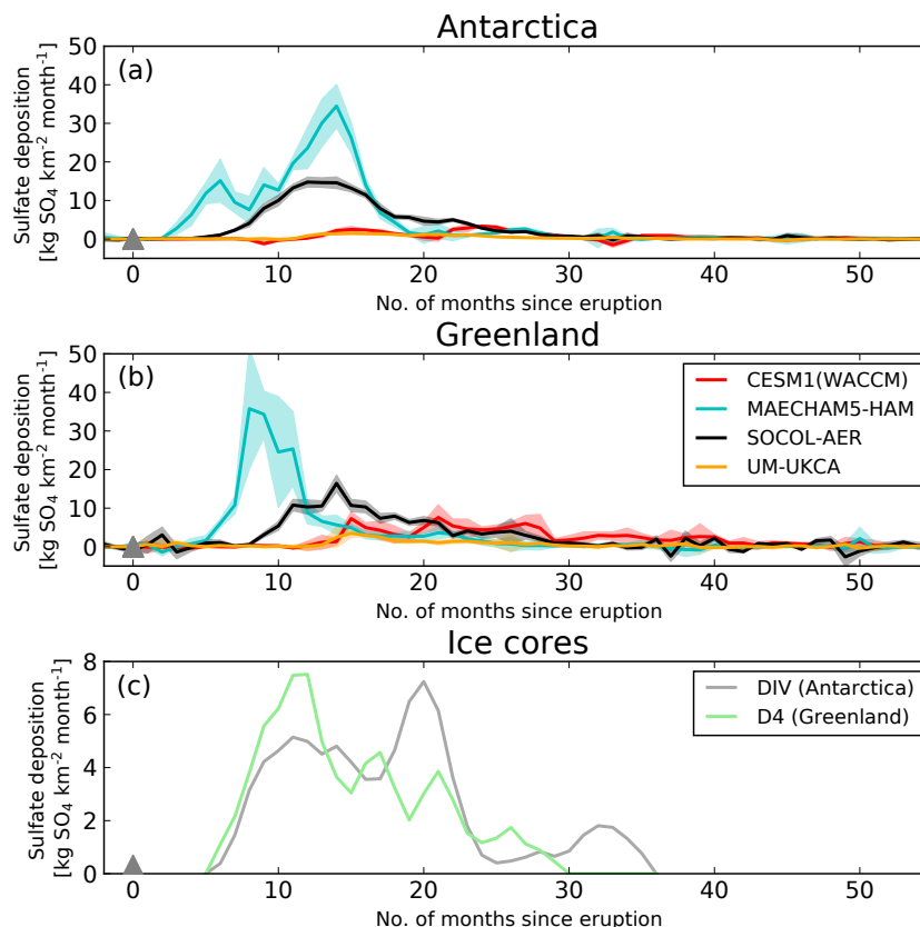
Figure 9. Simulated area-mean volcanic sulfate deposition ( \text{kgSO}_4 \text{ km}^{-2} \text{ month}^{-1} ) to the Antarctic ice sheet (top panel) and Greenland ice sheet (middle panel) for each model (colours). Each ice sheet mean is defined by taking an area-weighted mean of the grid boxes in the appropriate regions once a land–sea mask has been applied. Solid lines mark the ensemble mean and shading is 1 SD. In the bottom panel are deposition fluxes from two monthly CE2 resolved ice cores (DIV from Antarctica and D4 from Greenland). The scale is reduced in the bottom panel. The grey triangles mark the start of the eruption.
