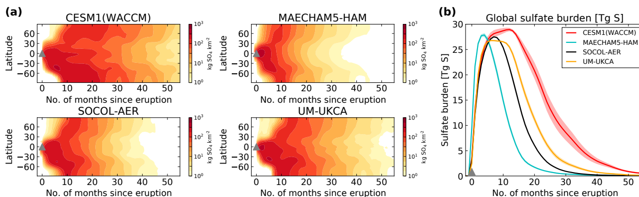
Figure 10. (a) Zonal mean atmospheric sulfate burdens in each model ( \text{kgSO}_4 \text{ km}^{-2} ) (ensemble mean) (b) global total atmospheric sulfate burdens ( \text{Tg S} ) in each model (colours). Ensemble means are shown by the coloured lines; shadings mark 1 SD. Sulfate burdens are monthly mean anomalies. The grey triangle marks the start of the eruption (1 April 1815).
