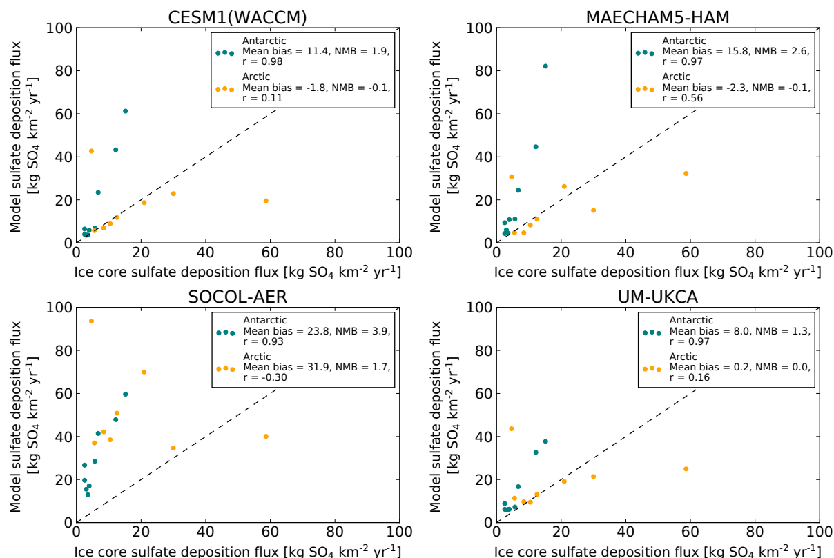
Figure 3. Scatter plots of preindustrial background ice core sulfate deposition fluxes vs. simulated preindustrial sulfate fluxes (kg SO 4 km -2 yr -1 ) in the Antarctic (teal points) and in the Arctic (orange points) for each model. Simulated values represent the grid box value where each ice core is located. The dashed line marks the 1 : 1 line. Included in the legends are the mean bias, normalized mean bias (NMB) and the correlation coefficient ( r ) for the Antarctic and Arctic.
