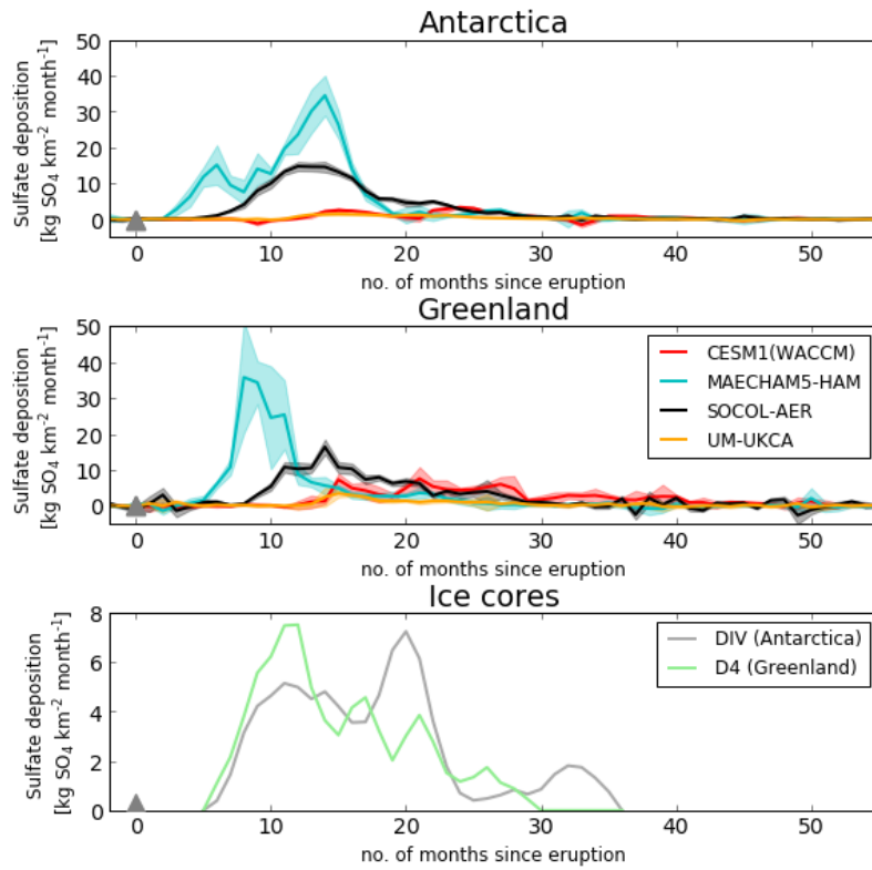
Figure 9: Simulated area-mean volcanic sulfate deposition [kg SO 4 km -2 month -1 ] to the Antarctic ice sheet (top panel) and Greenland ice sheet (middle panel) for each model (colours). Each ice sheet mean is defined by taking an area-weighted mean of the grid boxes in the appropriate regions once a land-sea mask has been applied. Solid lines mark the ensemble mean and shading is one standard deviation. In the bottom panel are deposition fluxes from two monthly resolved ice cores (DIV from Antarctica and D4 from Greenland). The scale is reduced in the bottom panel. The grey triangles mark the start of the eruption.
