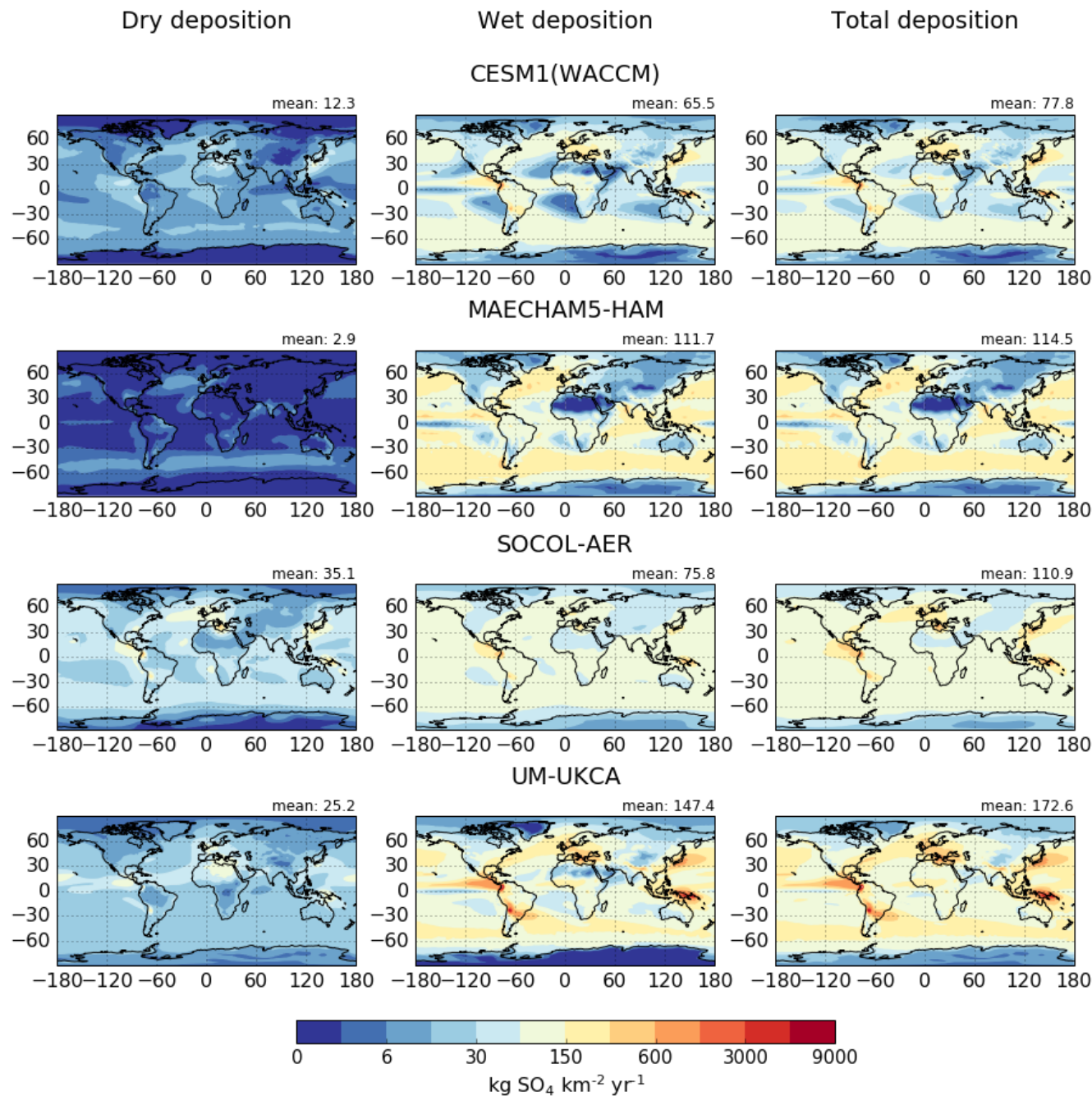
Figure 1: Pre-industrial background annual mean dry, wet and total (wet + dry) sulfate deposition fluxes [kg SO 4 km -2 yr -1 ] (left to right) for each model (top to bottom). The value shown in the top right-hand corner of each plot refers to the global mean sulfate deposition flux.
