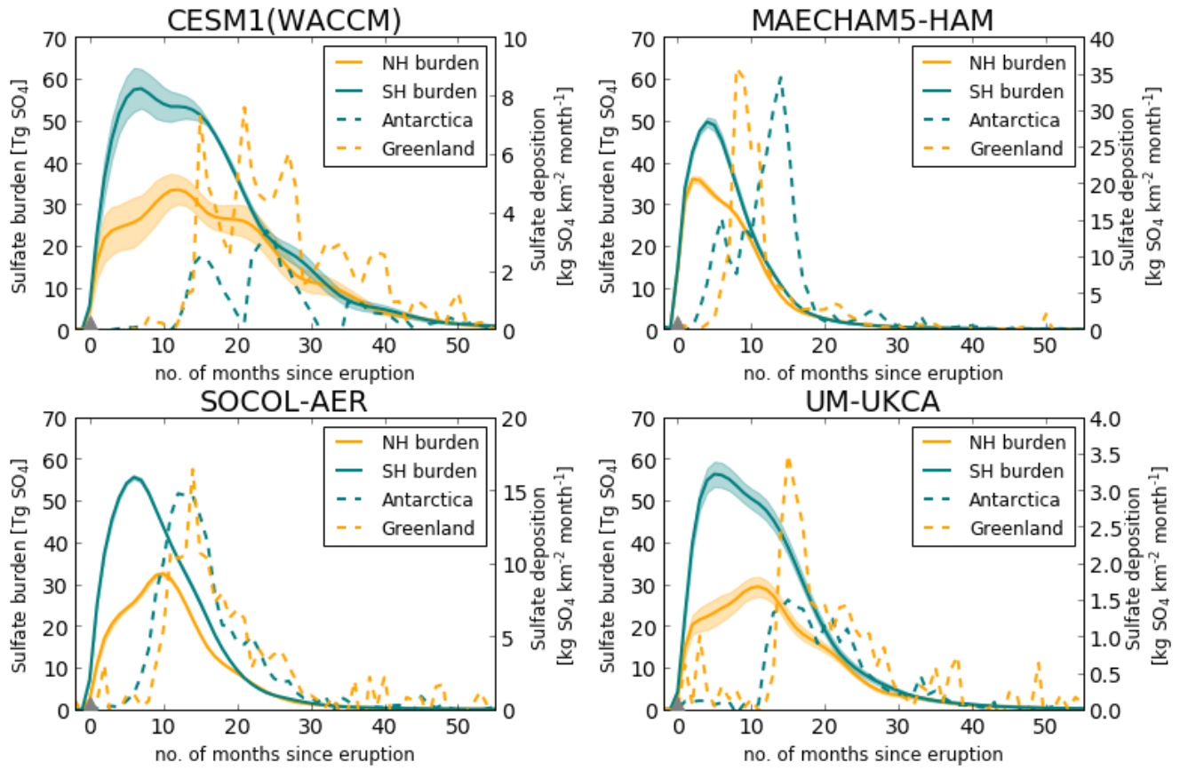
Figure 11: Hemispheric atmospheric sulfate burdens [Tg SO 4 ] (solid lines – ensemble mean, shading is one standard deviation) and area-mean ice sheet volcanic sulfate deposition as in Fig. 9 (dashed lines) [kg SO 4 km -2 month -1 ] for each model. The grey triangles mark the start of the eruption. There are different scales on each secondary y axis for ice sheet deposition.
