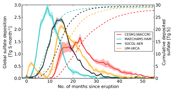
Figure 5. Global total volcanic sulfate deposition ( \text{Tg S month}^{-1} ) (solid lines – left axis) and global total cumulative deposited sulfate ( \text{Tg S} ) (dashed lines – right axis) for each model (colours). Ensemble mean is shown by the solid line; shading marks 1 SD. The grey triangle marks the start of the eruption (1 April 1815).
