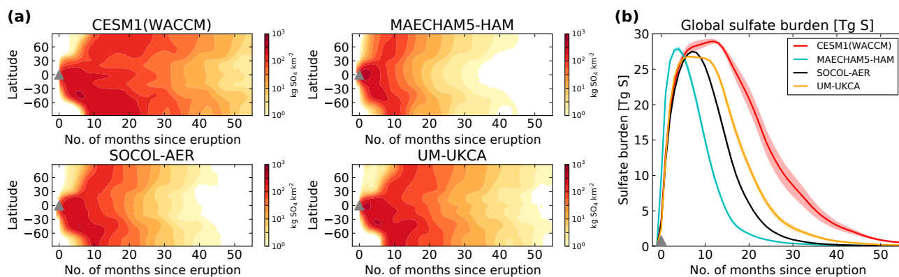
Figure 10. (a) Zonal mean atmospheric sulfate burdens in each model ( \text{kg SO}_4 \text{ km}^{-2} ) (ensemble mean) (b) global total atmospheric sulfate burdens (Tg S) in each model (colours). Ensemble means are shown by the coloured lines; shadings mark 1 SD. Sulfate burdens are monthly mean anomalies. The grey triangle marks the start of the eruption (1 April 1815).
