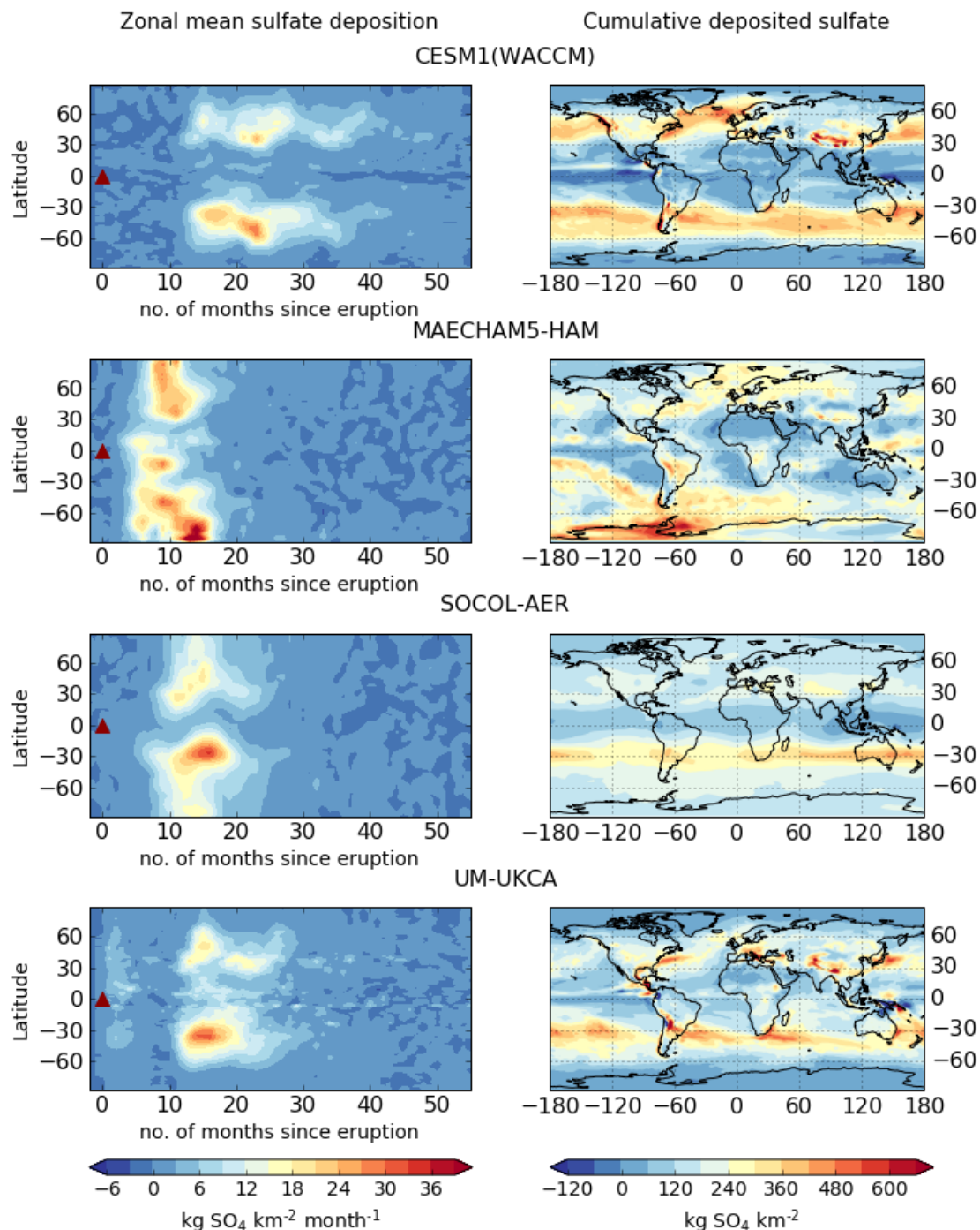
Figure 34: Zonal mean monthly-mean volcanic sulfate deposition [ \text{kg SO}_4 \text{ km}^{-2} \text{ month}^{-1} ] (left) and cumulative deposited sulfate [ \text{kg SO}_4 \text{ km}^{-2} ] (right) for each model (ensemble mean). The red triangle marks the start of the eruption (1 April 1815). Volcanic sulfate deposition is calculated as the difference in total sulfate deposition (wet + dry) between the perturbed and control simulations and this anomaly is summed over the ~5 years of simulation to produce the cumulative sulfate deposition maps (right column).
