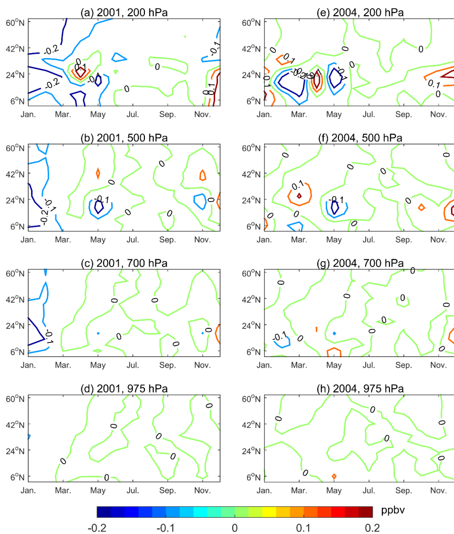
Figure S1. The differences of imported African ozone over Asia between the 2005 and the 2001 datasets (1 st col.) and between the 2005 and the 2004 dataset (2 nd col.). The
