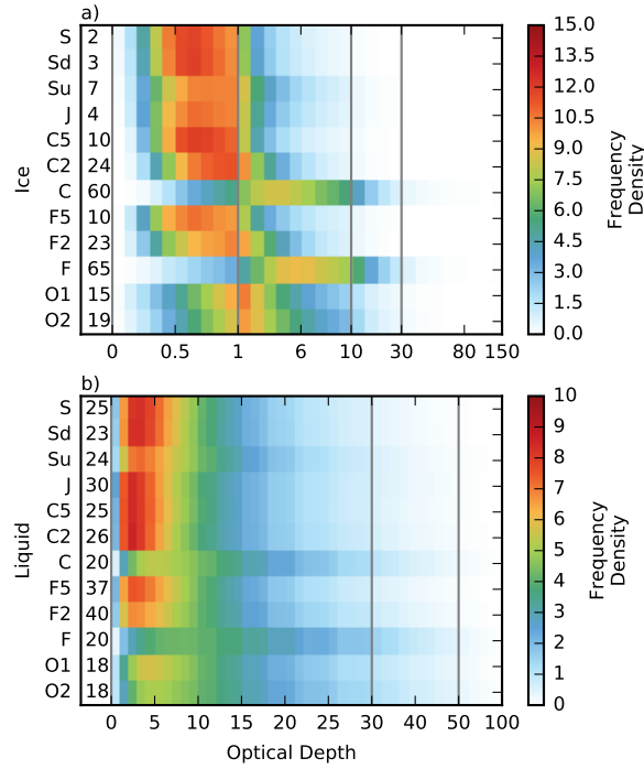
Figure 6. The mean normalised MODIS collection 6 cloud optical depth (COD) distribution for each of the regimes, showing clouds classified as a) ice-phase and b) liquid-phase separately. The bins are taken from the MODIS level 3 daily product, vertical lines indicate a change in bin width. The frequency density is normalised by the bin width and sums to one within each regime. The numbers along the right-hand edge of each plot show the percentage occurrence of valid retrievals within that regime (analogous to a cloud fraction). Note the different scale for the two plots.
