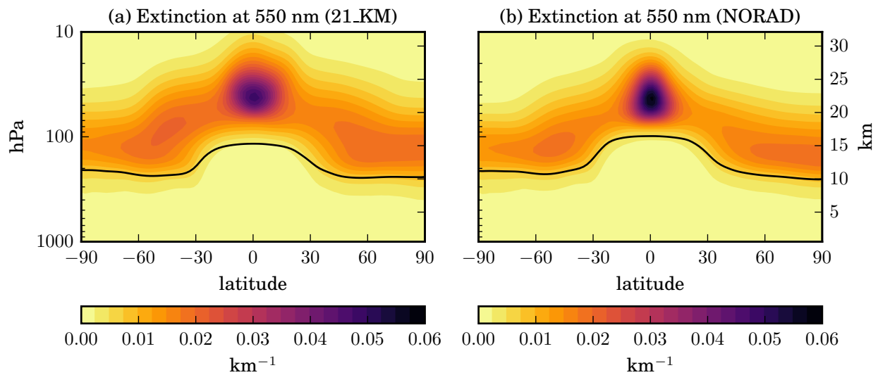
Figure 14. Latitude-height cross-section of the zonal and annual mean distribution of the aerosol extinction coefficient ( \text{km}^{-1} ) at 550 nm for equatorial stratospheric aerosol sulfur injections at 21 km from (a) a simulation with radiatively interactive aerosol (21_KM) and (b) a simulation with non-radiatively interactive aerosol (NORAD).
