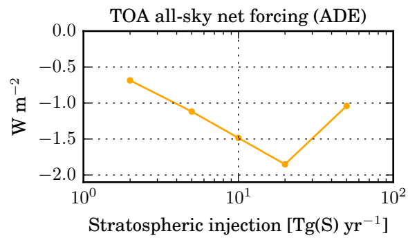
Figure 5. Global mean instantaneous net radiative forcing (aerosol direct effect = ADE) at the top of the atmosphere (TOA) in \text{W m}^{-2} for the x\_TGS experiments with different injection rates.
