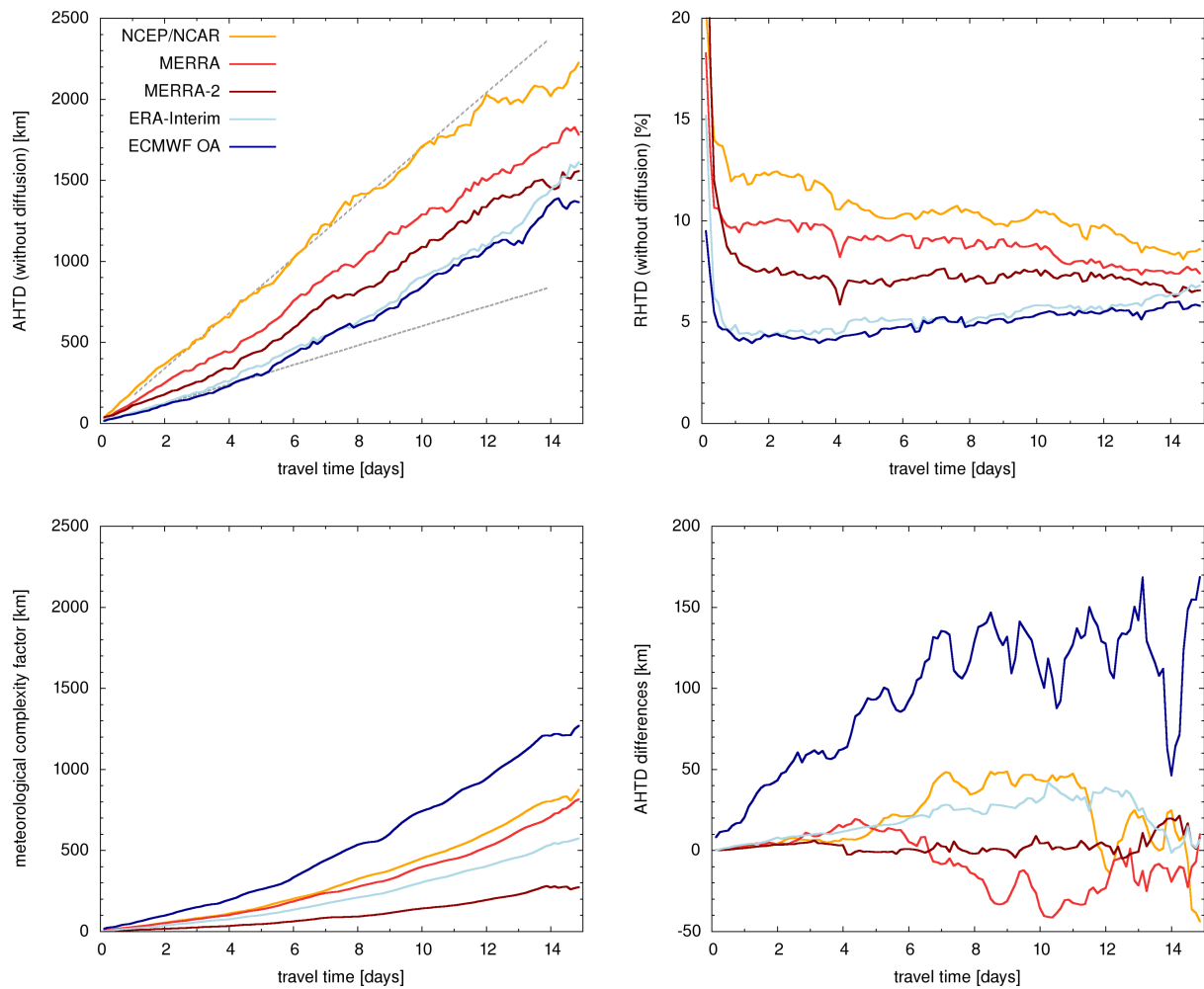
Figure 9. Horizontal transport deviations of simulated and observed balloon trajectories for different meteorological analyses (top). Dotted gray lines represent AHTD growth rates of 60 and 170 km day -1 . Also shown are the meteorological complexity factor for dispersion simulations (bottom, left) and the AHTD differences that are introduced by adding diffusion (bottom, right).
