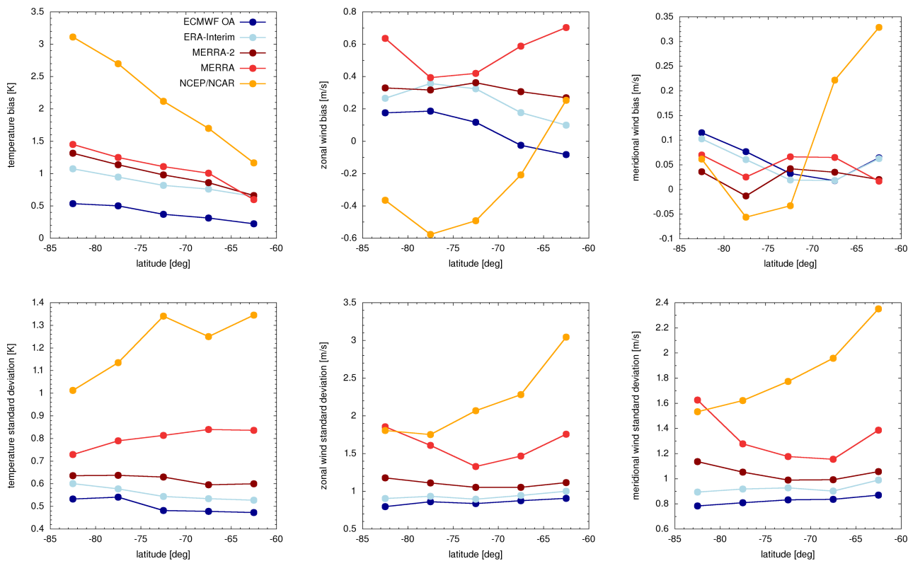
Figure 5. Bias and standard deviations of temperature and horizontal winds of meteorological analyses minus Concordiasi balloon data at different latitudes.
