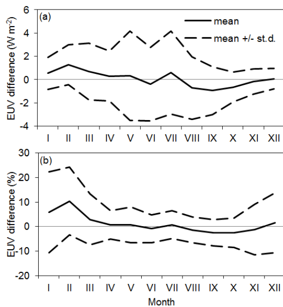
Figure 1. The mean (a) absolute and (b) relative differences between the observed and modeled EUV radiation intensities and their standard deviations (st.d.) at the Hradec Králové observatory in the period 2005–2013.
