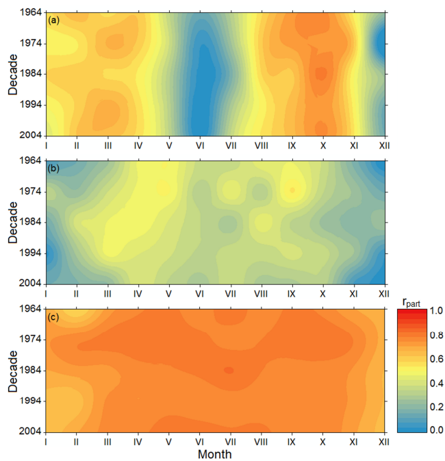
Figure 3. Partial correlation coefficients ( r_{\text{part}} ) of the effects of (a) SZA, (b) TOC, and (c) cloud cover on the daily doses in individual months and decades; the decades are labeled only by their initial years.
