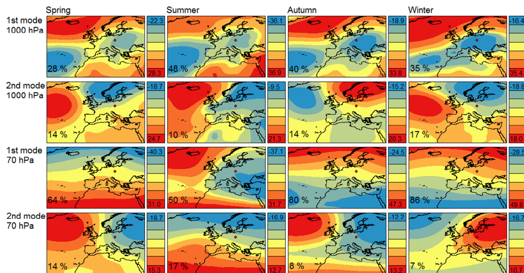
Figure 5. The values of the first and second PCA modes of the 1000 hPa and 70 hPa geopotential heights for the days with EUV_{90+} in spring, summer, autumn, and winter (represented by the color legend on the right). Variability explained by each of the modes is indicated by the relative value in the bottom-left corner. The red dot marks the location of the Hradec Králové observatory.
