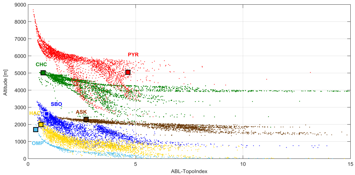
Figure 6: a) ABL-TopoIndex, b) drainage basin for convection, c) hypsometric percentage of the station elevation, d) hypsometric percentage of the station elevation minus the 50% hypsometry, e) local slope in a circle of 10 km radius centered on the station, f) gradient in elevation as a function of the domain size for some European high altitude stations.
