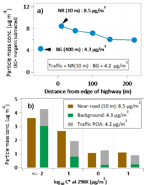
Figure 8: (a) An example of measured upwind (background) and downwind concentrations of OA mass loading as a function of distances from the highway. (b) Distributions of OA mass loading (particle-phase only) as measured at 10 m downwind (brown bar) and apportioned to vehicle emissions (grey) and background (green) volatility distributions using distributions from May et al. (2013a) and fits to downwind (220 m) TD data, respectively.
