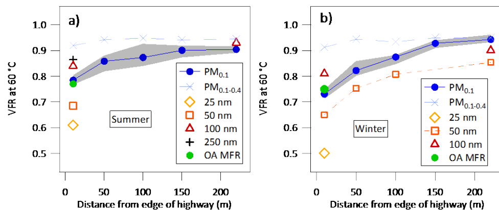
Figure 1: Campaign-average downwind evolution of volume fraction remaining (VFR) of near-road particles after heating at 60 °C in a TD ( R_t = 30 s) during (a) summer, and (b) winter. VFR of size-selected particles (e.g., 25, 50, 100, 250 nm) obtained from V-TDMA measurements. VFR of PM_{0.1} and PM_{0.1-0.4} estimated from integrated SMPS volume between 10-100 nm and 100-400 nm, respectively. OA MFR was measured using a TD/ACSM system ( R_t = 30 s) in the near-road trailer. The shaded area represents interquartile range of all measurements for each season.
