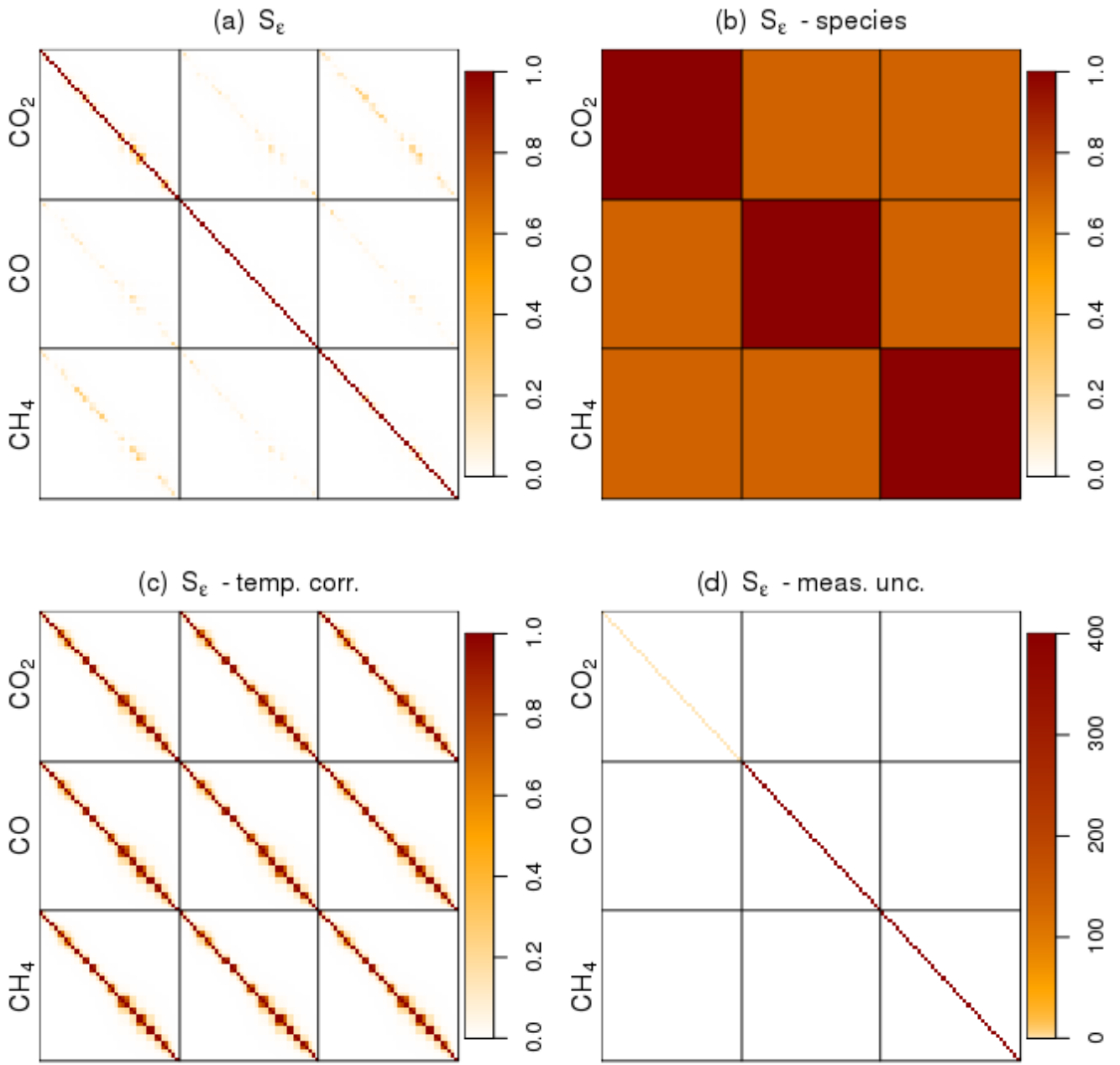
5 Figure 3: Model-data mismatch correlation matrix (a) used in the multi-species inversion, species correlation matrix S_s (b), temporal correlation matrix S_t (c) and squared measurement uncertainty (d). Note that the measurement uncertainty is expressed in ppm for CO 2 and ppb for CO and CH 4 . Each matrix has the same dimensions (1098x1098) reflecting the length of the observation vector, but here only the data of July are plotted to increase visibility. The gray lines indicate different species in the observation vector ('blocks'), ordered as follows from top to bottom and from left to right: total CO 2 , CO and CH 4 . In the single-species inversion, the correlation value in the off-diagonal 'blocks' of matrix (b) is set to zero. The structure in S_s in (c) is a result of the uneven temporal distribution of the observations within the month.
