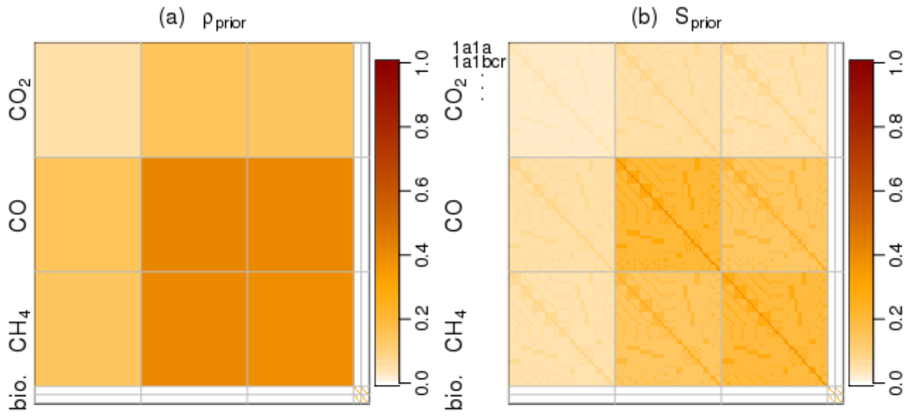
Figure 4: The final rescaling matrix \rho_{\text{prior}} (a) and the prior error covariance matrix S_{\text{prior}} (b). Note that \rho_{\text{prior}} can be defined as the element-wise ratio of S_{\text{prior}} and C_{\text{prior}} .
