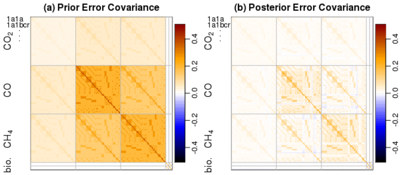
Figure 6: Prior error covariance matrix (left) and corresponding posterior error covariance matrix (right).
