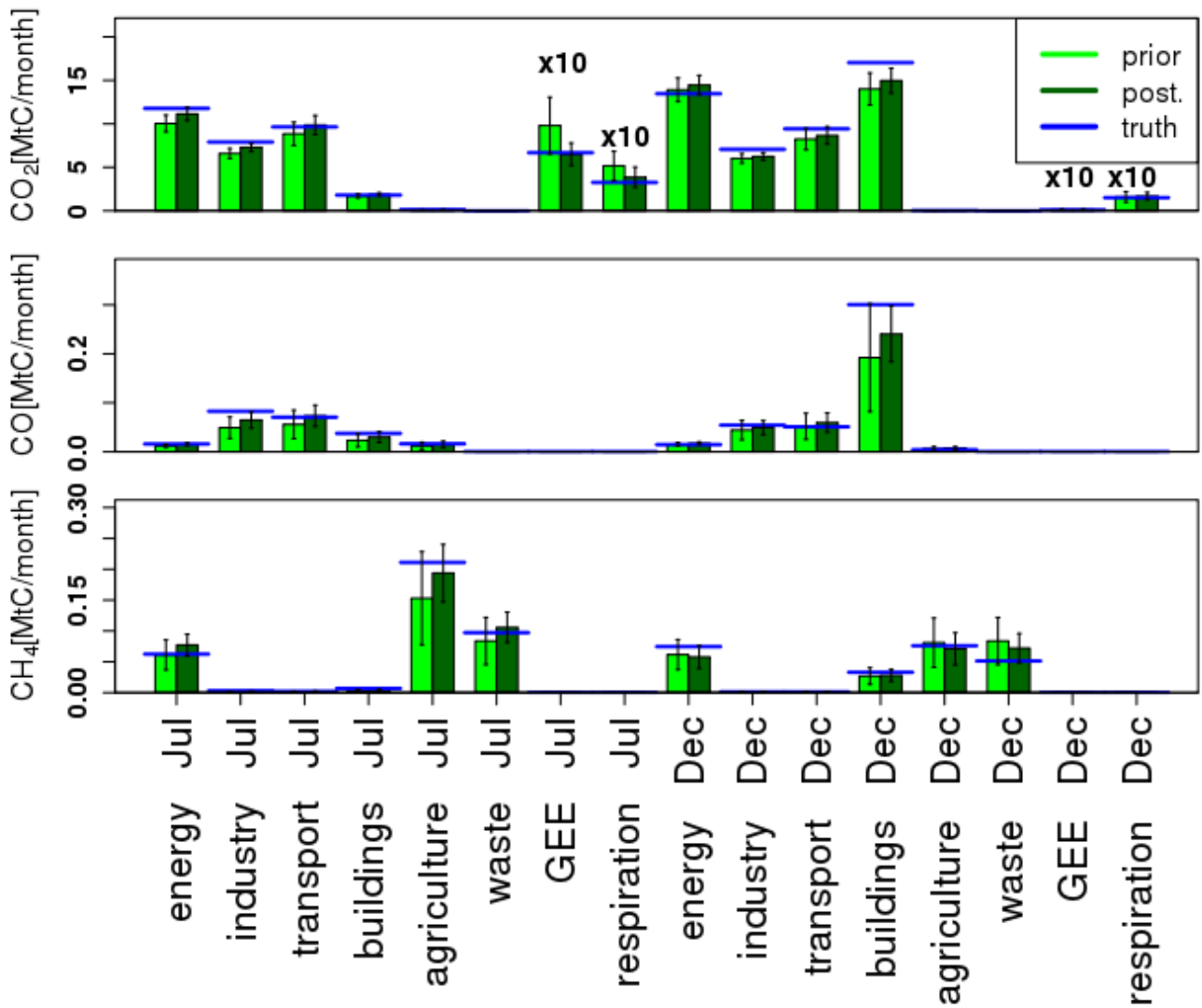
Figure 8: Prior, posterior and true (pseudo-data) fluxes in physical units aggregated for different emission sectors. Absolute values of biosphere-atmosphere exchange fluxes of CO 2 are included in (b), but scaled down by a factor of 10. Note that, as the true fluxes are the result of a random perturbation of the prior, they do not describe an actual situation in the physical world. So, for example, the fact that the true value of CO for transport in July is higher than the same value in December should not be surprising.
