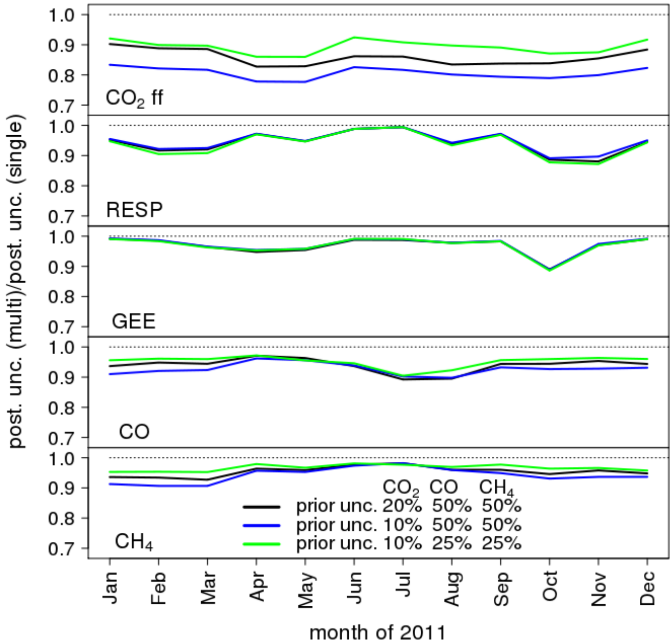
5 Figure 10: Benefit of a multi-species inversion over the corresponding single-species (dotted line) per different species per months of the year. The benefit has been tested for the three different cases of Table 3. Note that CO 2 refers to fossil fuel emissions only, and RESP and GEE refers to the biospheric fluxes.
