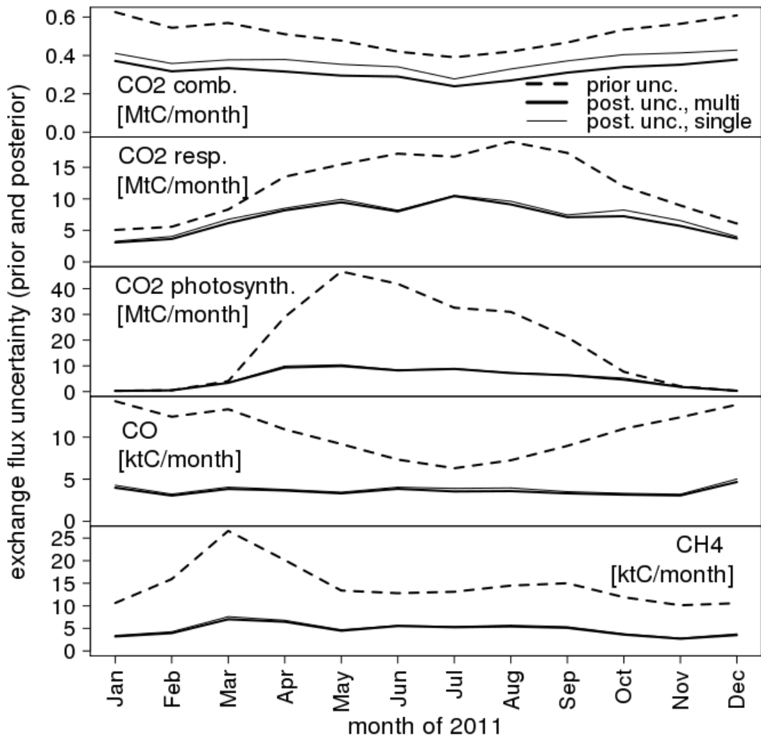
5 Figure 9: Comparison between prior and posterior monthly uncertainties for the five tracers. The posterior uncertainty is plotted for both the multi-species inversion, accounting for inter-species correlations, and the single-species inversion, in which all of the species are independent. Both prior and posterior uncertainty are expressed in physical units. The spike in the prior methane uncertainty estimate for the month of March depends on the emission inventory and is related to the cycle of agricultural activities.
