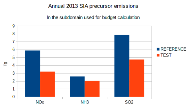
Figure 11. Annual emissions of SIA precursors, \text{NO}_x , \text{NH}_3 and \text{SO}_2 for the year 2013 computed over the budget domain in the reference simulation in blue and the sensitivity test in red.
