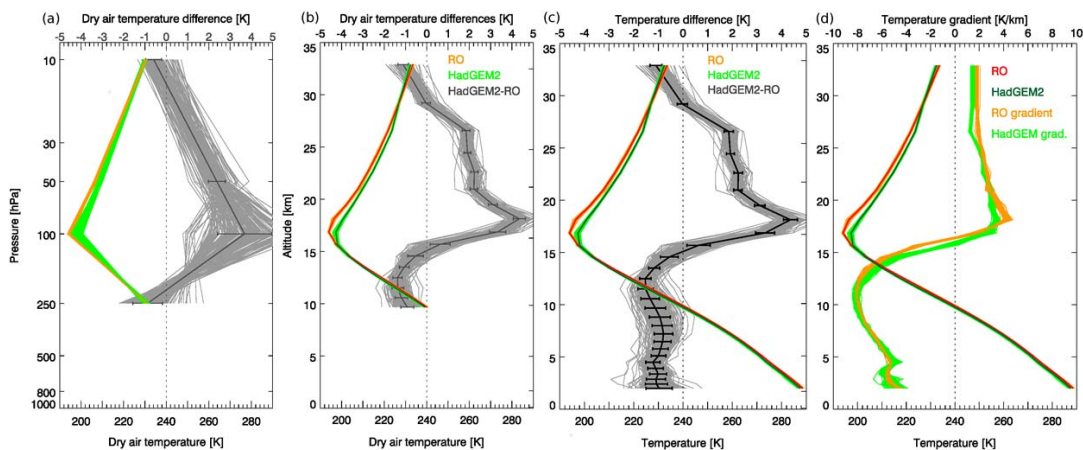
Figure 4. Comparison of HadGEM2-A model data to RO observations for all classes ( \omega_{500} and T_{2m} ) in the tropics in terms of collocated temperature profiles and temperature difference profiles of HadGEM2-A minus RO (lower axes depict absolute values, upper axes differences to RO). Shown are dry temperature (see Sect. 2.1) at coarse vertical resolution for four pressure levels (a), dry temperature at high vertical resolution for altitude levels (b), as well as physical temperature at high vertical resolution (c) and corresponding temperature gradients (d).
