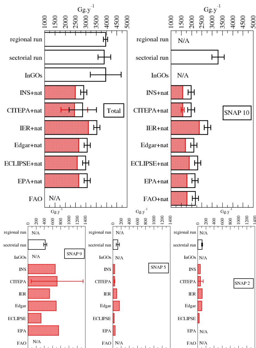
Figure 9. CH_4 yearly emissions (in Gg\ CH_4 ) in France for this study and the other studies/inventories listed in Table 5. "Total": the inventories including only anthropogenic emissions (in red) are summed-up with the natural emissions by wetlands and termites. For these totals (black bars), the error bars (in black) are obtained from the range on wetland emissions (Table 5) combined with the uncertainty on anthropogenic emissions (in red), when available i.e. only for CITEPA (Table 5). The CITEPA provides uncertainties only for the main emitting sectors so that the error bar on the total emissions is under-estimated. "SNAP10": the inventories including only anthropogenic emissions (in red) are summed-up with the natural emissions by wetlands and termites. Only the CITEPA provides an uncertainty (in red), which is combined to the range on wetland emissions to obtain the error bar on the whole sector (in black). Other sectors: only the CITEPA provides an uncertainty for these sectors. N/A = not-available or the definition of sectors/activities does not match those of SNAPs.
