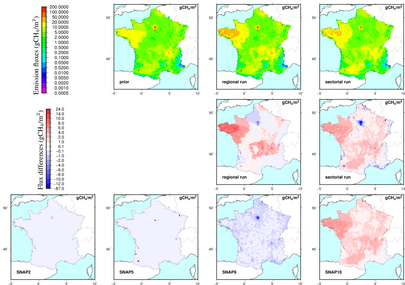
Figure 4. Annual median CH_4 emission fluxes in gCH_4/m^2 in France (top, prior from IER, inferred fluxes from the regional and sectorial runs); differences inferred minus prior (middle) for the regional and sectorial runs; details for the sectorial run (bottom): differences inferred minus prior for the 4 sectors which are actually seen, SNAPs 2, 5, 9 and 10.
