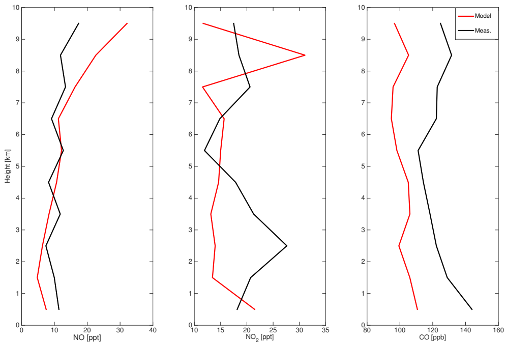
Figure S 3. Vertical profile for median modeled (red) and measured (black) NO, NO 2 , and CO for Honolulu based INTEX-B flight data binned by kilometer
