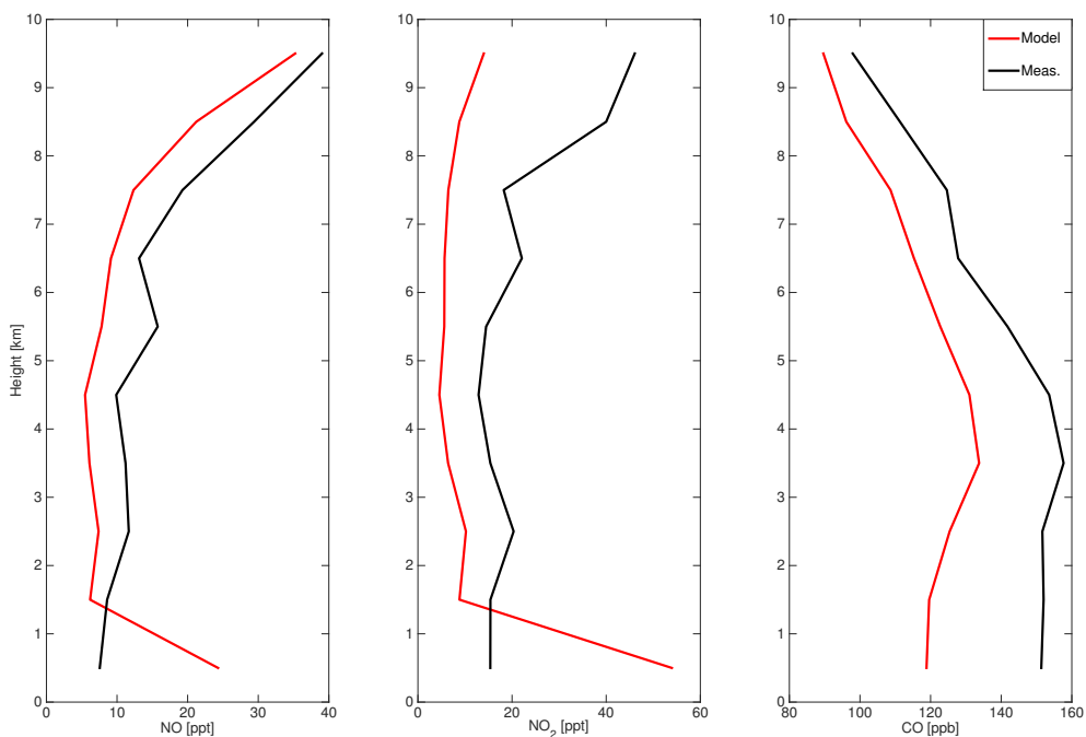
Figure S 4. Vertical profile for median modeled (red) and measured (black) NO, NO 2 , and CO for Anchorage based INTEX-B flight data binned by kilometer
