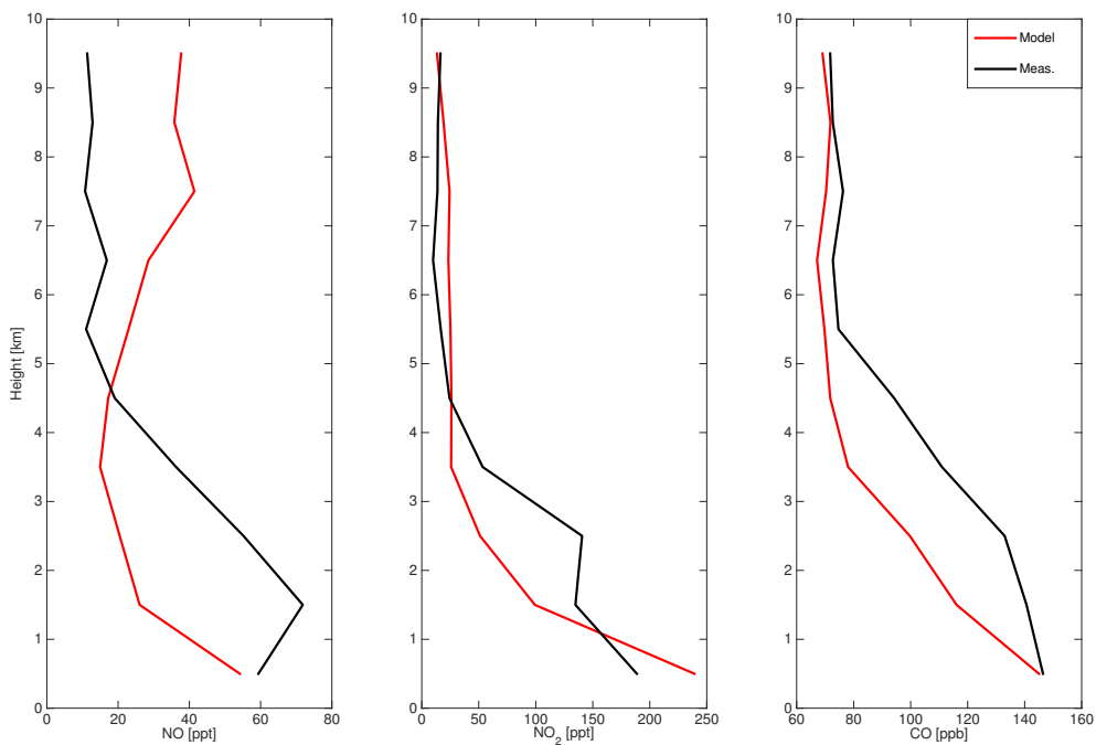
Figure S 2. Vertical profile for median modeled (red) and measured (black) NO, NO 2 , and CO for Houston based INTEX-B flight data binned by kilometer
