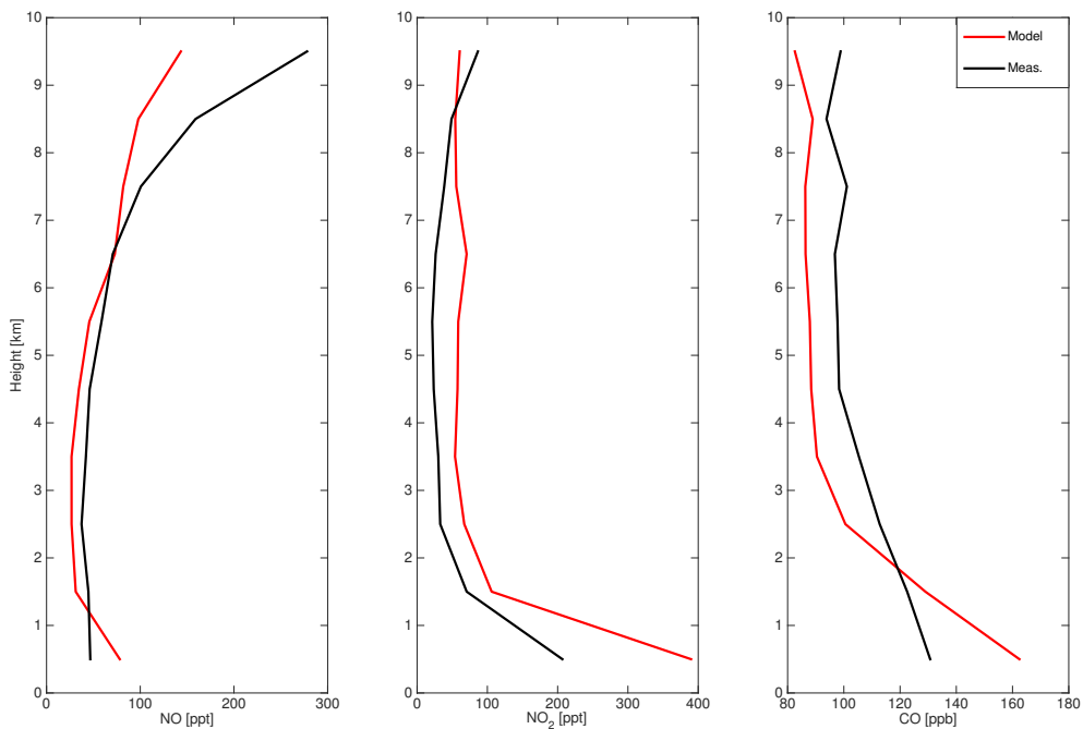
Figure S 1. Vertical profile for median modeled (red) and measured (black) NO, NO 2 , and CO for INTEX-A flight data binned by kilometer.
