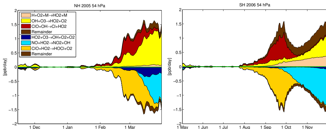
Figure 10. Vortex-averaged chemical reaction rates of reactions changing HO 2 for the Arctic winter 2004/2005 (left) and the Antarctic winter 2006 (right) at 54 hPa to illustrate HO x partitioning. Production reactions are shown positive and are separated by a line in the legend from the loss reactions, which are shown negative. The net change of HO 2 is shown as a green line.
