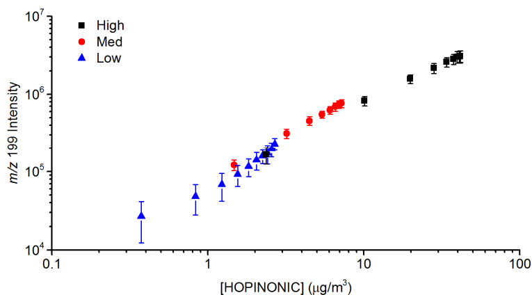
Figure 8: Correlation between MS intensity and MCM mass across three different experiments for OH-pinonic acid.
