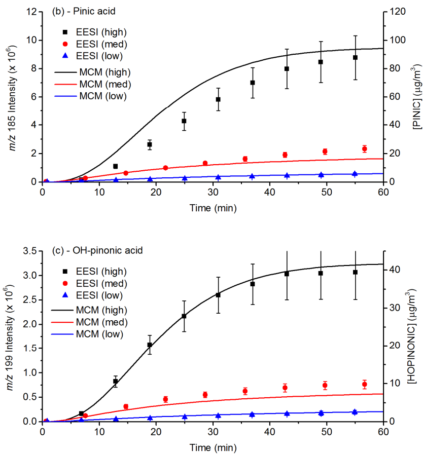
5 Figure 7: Comparison between EESI-MS intensities (left y-axis) and MCM simulated concentrations (right y-axis) for (a) pinonic acid, (b) pinic acid and (c) OH-pinonic acid during chamber experiments with different [\alpha\text{-pinene}]_0 . MS intensities are absolute, following averaging and blank subtraction. The measurements and model agree closely both in terms of the time dependence of product formation and the relative yields under different reaction conditions.
