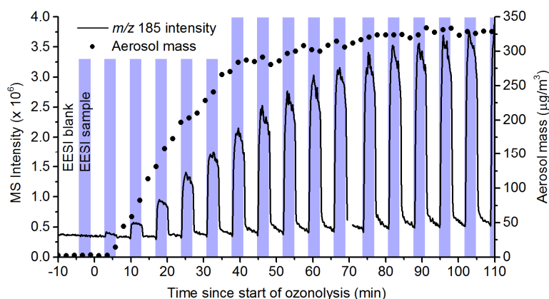
10 Figure 5: Left y-axis: Intensity of m/z 185.0819, corresponding to pinic acid, after the start of an \alpha -pinene ozonolysis experiment. Right y-axis: Mass concentration of aerosol in the chamber. The measurements were made using the new EESI-MS batch sampling system (Figure 1). Blue bands correspond to 15 sampling of chamber air from the reservoir volume (3.5 minutes) while the blanks in between correspond to clean air flushing (3.5 minutes). The MS discontinuity around 70 minutes corresponds to refilling of the primary EESI solvent syringe.
