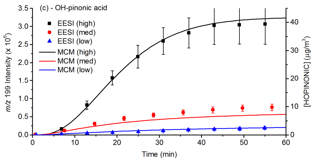
Figure 8: Comparison between EESI-MS intensities (left y-axis) and MCM simulated concentrations (right y-axis) for (a) pinonic acid, (b) pinic acid and (c) OH-pinonic acid during chamber experiments with different [\alpha\text{-pinene}]_0 . MS intensities are absolute, following averaging and blank subtraction. The measurements and model agree closely both in terms of the time dependence of product formation and the relative yields under different reaction conditions.
