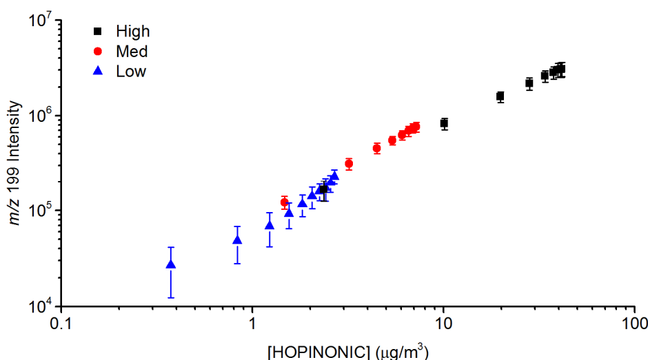
Figure 9: Correlation between MS intensity and MCM mass across three different experiments for OH-pinonic acid.
