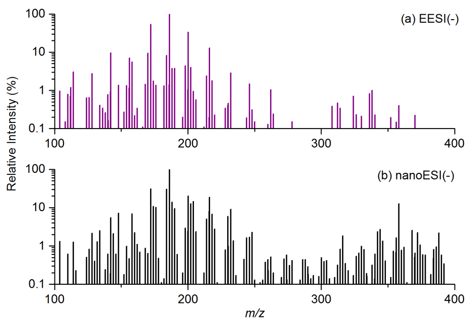
Figure 5: Mass spectra obtained during the dark ozonolysis of \alpha -pinene under “medium” conditions (Table 1) using (a) online EESI-MS in negative ionisation mode and (b) nanoESI-MS of SOA filter extracts. The online MS was acquired and the filter collected 1 hour after the start of ozonolysis in the chamber. The spectra are very similar in the monomer region (< 250 Da), but the oligomers detected are more numerous and possess slightly higher molecular weights in the nanoESI(-) spectrum.
