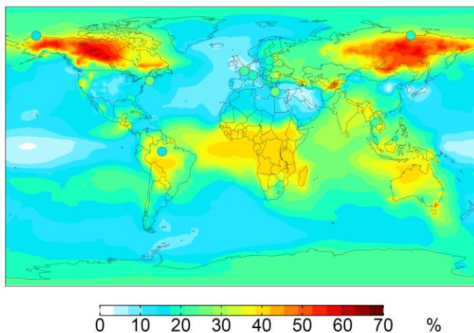
Figure 7. Global distribution of simulated BrC absorption contribution to total aerosol absorption at the surface for 2014. Results are from the Modified_Age simulation. The circles show the retrieved results from multiple-wavelength absorption measurements at 8 surface sites (see Section 5.1 for details).
