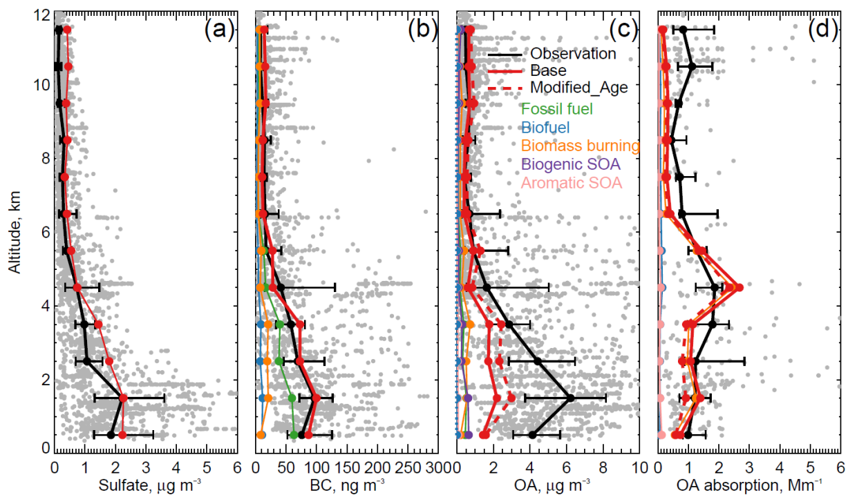
Figure 2. The median vertical profile of (a) sulfate, (b) BC, (c) OA mass concentration and (d) OA absorption, shown in 1 km bins, from the DC-8 aircraft measurement during DC3 campaign in the region shown in Figure 1. Observations (black) are compared to the Base simulation (red) and source-specific contributions to that simulation, as well as to the optimized Modified_Age simulation (red dashed). Error bars show the 25 th and 75 th percentiles of measurements in each vertical bin. Gray points show the original measurements (1-minute averaged values for a, b and c, 5-minutes averaged values for d). The ranges of x-axes are set to emphasize the vertical profile, so several data points higher than the maximum values of x-axes are not shown. Details regarding the model simulations of Base and Modified_Age can be found in Sections 3.2 and 4.1.
