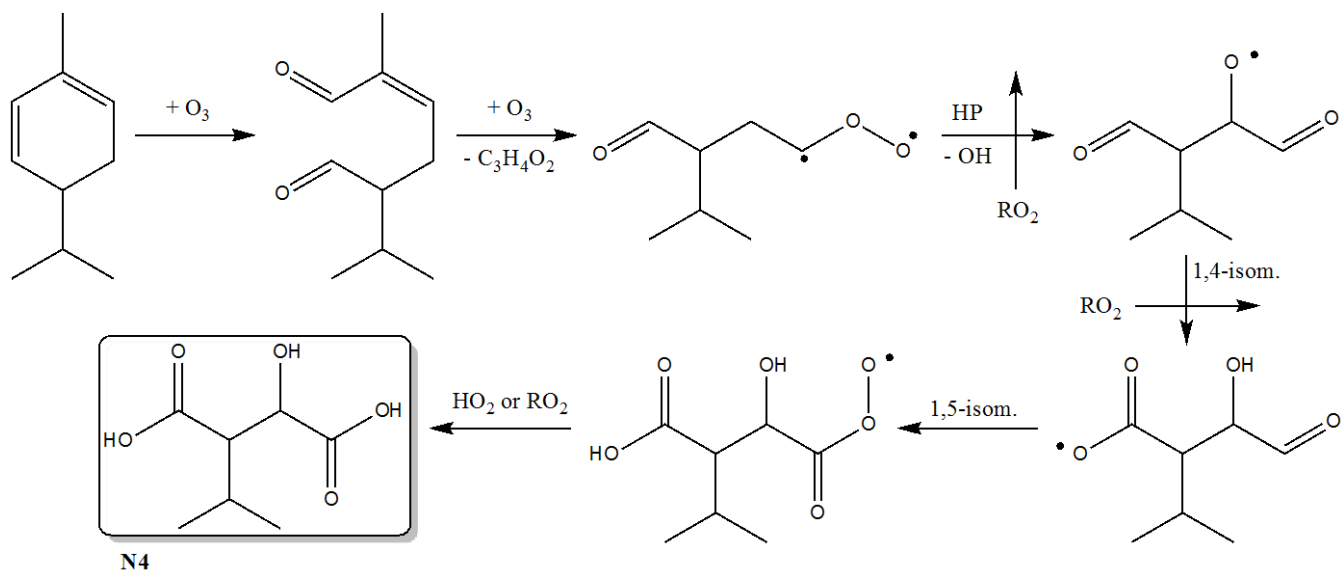
Figure 3: Proposed formation mechanism of compound N4. N5 is formed through an analogous mechanism starting with initial attack of ozone at the more substituted double bond. Vertical arrow with \text{RO}_2 denotes a peroxy radical self-reaction to form an alkoxy radical.
