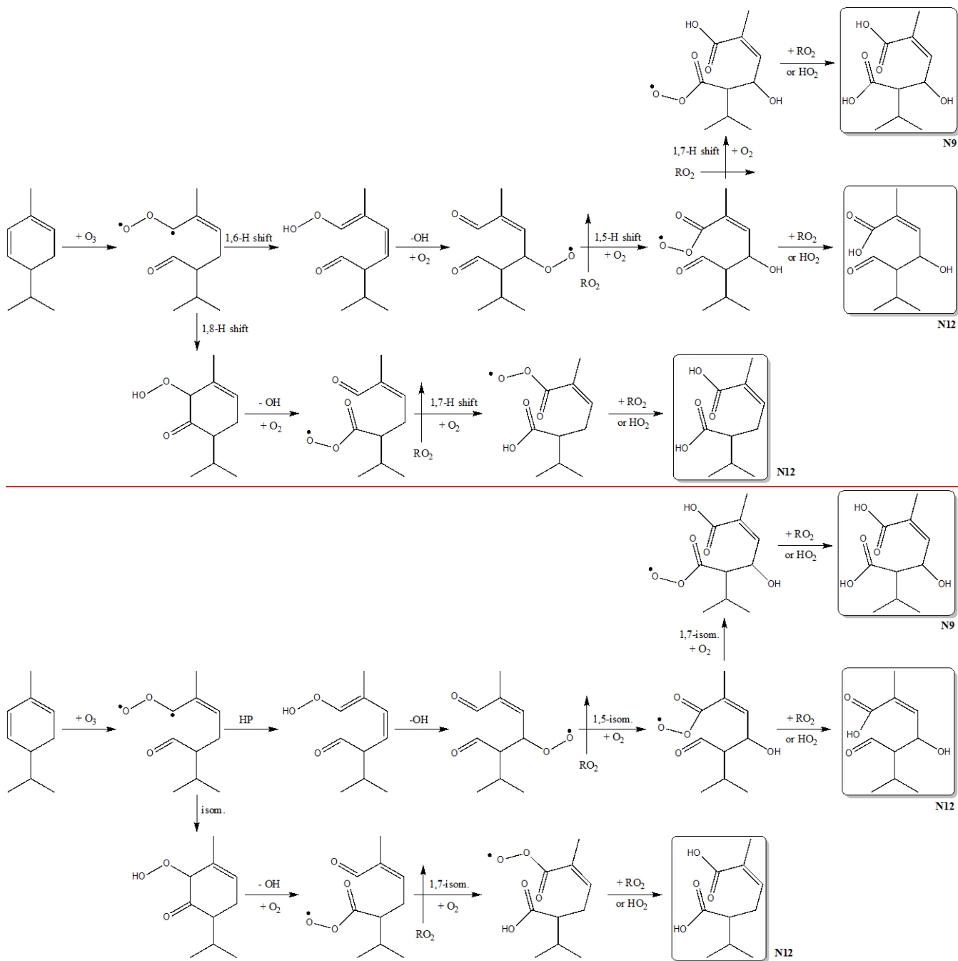
Figure 4: Formation mechanisms of compounds N9 and N12. Perpendicular arrows with RO_2 denote peroxy radical self-reactions to form an alkoxy radical.
