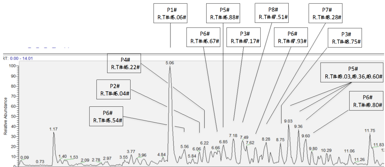
Figure 5: Positive ionisation mode chromatogram of SOA generated from the ozonolysis of \alpha -phellandrene (experiment 9). Major positive mode ionisation peaks detected across all experiments (Table 3) are labelled.
