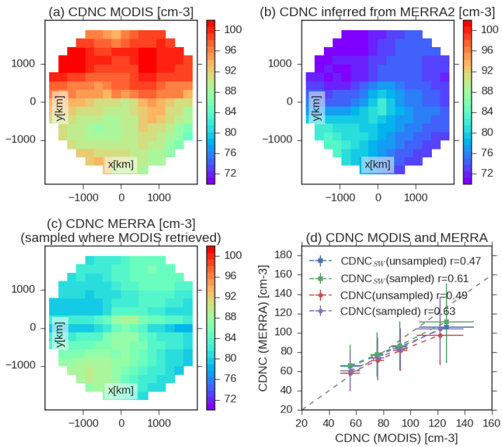
Fig. 4 Cyclone composited CDNC (a) retrieved by MODIS, (b) inferred from MERRA2, (c) inferred from MERRA2, but sampled so that failed retrievals from MODIS are not used in calculation of the mean composite from MERRA2. Figure (d) Shows the covariability between MERRA2-inferred and MODIS-retrieved cyclone-mean and southwest quadrant (poleward-oriented) CDNC (CDNC SW ). The CDNC from MERRA2 is plotted on the y-axis and is shown binned by MODIS CDNC. Error bars show one standard deviation over each bin. The correlation between the CDNC (and CDNC SW ) from MODIS and from MERRA2 for all cyclones in the observational record is noted in the legend. CDNC (and CDNC SW ) from MERRA2 is calculated when all data is used (unsampled) and when it is sampled to correspond to MODIS.
