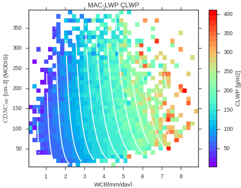
5 Fig. 15 The cyclone-mean CLWP in units of g/m^2 of liquid water observed by MAC-LWP binned as a function of WCB moisture flux and the CDNC_{SW} retrieved by MODIS. Data is binned into equal size bins for the purpose of visualizing the data record. White lines show contours of constant CLWP as predicted by Eq. 1 and the coefficients listed in Table 2. The dependence of CLWP on CDNC_{SW} inferred from MERRA2 is shown in Fig. S12.
