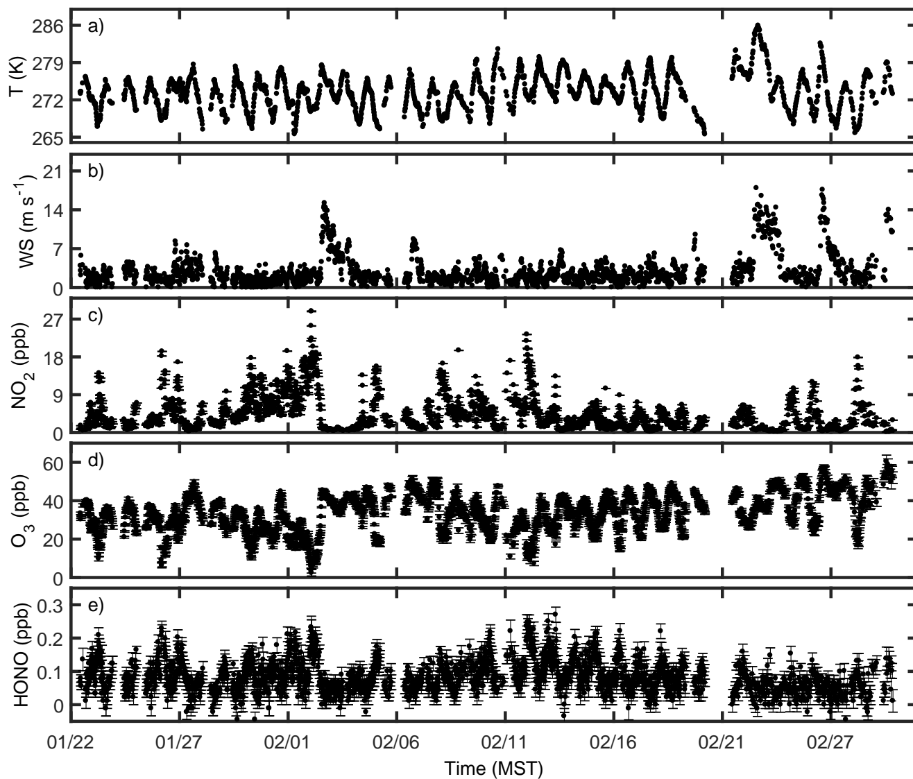
Figure 4. Overview of meteorological parameters (a,b) and mixing ratios of (c) \text{NO}_2 , (d) \text{O}_3 , and (e) \text{HONO} observed on the lower light path throughout the study.
