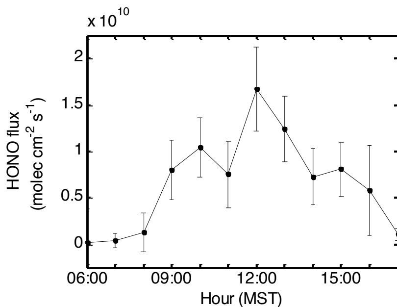
Figure 7. Sunny days hourly average vertical HONO fluxes derived from the HONO gradient observations during UBWOS 2012
