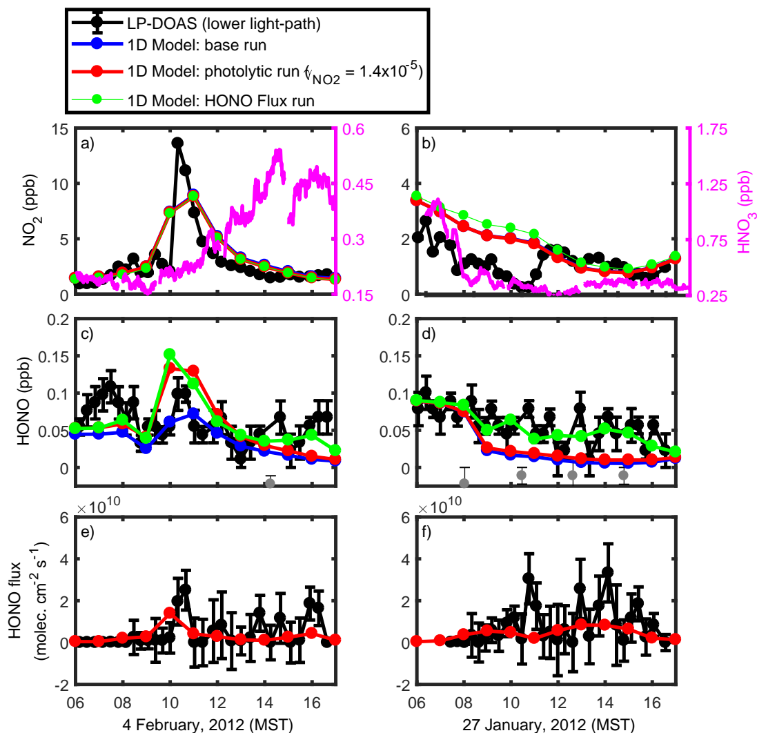
Figure 9. Comparison of modeled and measured \text{NO}_2 (a, b), HONO (c,d), and HONO flux (e,f) for 4 February 2012 (left panels: a, c, and e) and 27 January 2012 (right panels: b, d, and f). LP-DOAS lower light path \text{NO}_2 and HONO mixing ratios and errors are shown in black. We excluded a number of outliers (marked in grey) from the HONO analysis. These outliers are a consequence of problems with the DOAS analysis procedure for these specific measurement. Modeled \text{NO}_2 and HONO mixing ratios in the lower light path interval using the RCAT 8.2 base run are shown in blue, HONO flux run results are shown in green, and photolytic run results are shown in red (with \text{NO}_2 uptake coefficient of 1 \times 10^{-6} for 4 February and 1.4 \times 10^{-5} for 27 January). \text{HNO}_3 mixing ratios measured by NOAA are shown in magenta lines in the upper panels plots (a and b).
