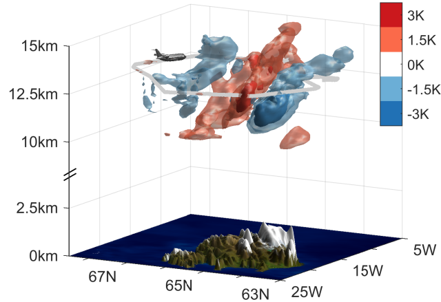
Figure 2. Tomographic retrieval of the temperature field for the research flight on January 25, 2016, over Iceland. Shown are isosurfaces of the temperature residual. The grey line around the retrieved 3D pattern indicates the flightpath.
