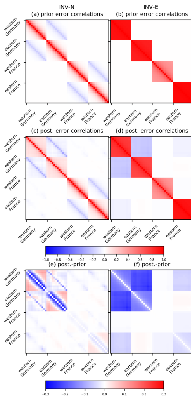
Figure 6: The correlation structure in the prior (first row) and posterior (second row) uncertainties in monthly regional FFCO 2 emissions for the four Germany and France regions using the NET43 network and 2-week sampling for INV-N (first column) and INV-E (second column) inversions, as well as their differences (third row). The x and y axes cover all the control region-months iterating through region first and months second (the blocks of pixels in each matrix). For clarity, we group these correlations into four regions and organize them for each region according to month indices.
