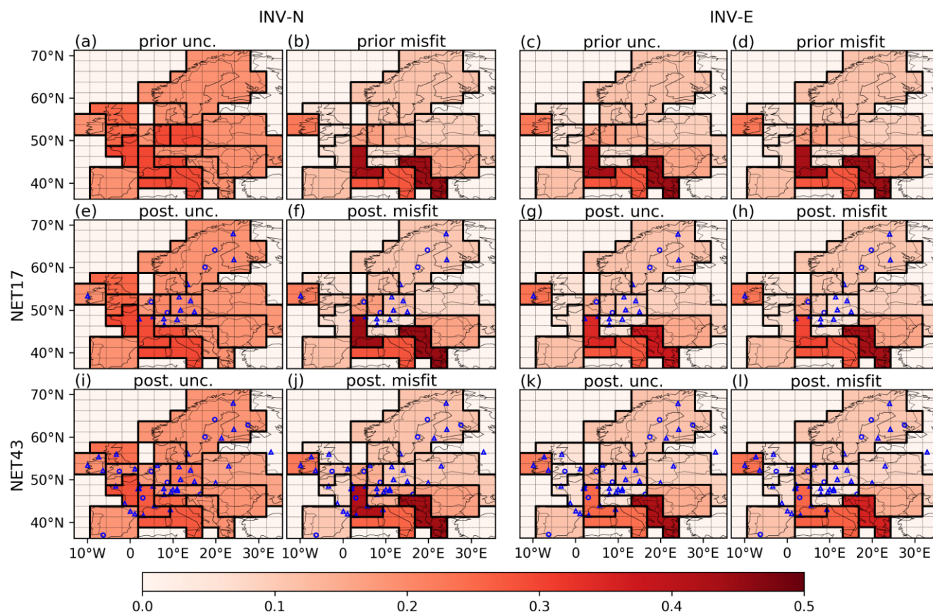
855 Figure 5: Average monthly relative prior and posterior uncertainties and misfits of FFCO 2 emissions over regions delineated by black lines, using the NET17 and NET43 networks and 2-week sampling for INV-N (first and second columns) and INV-E (third and fourth columns) inversions. First row shows the relative prior uncertainties and misfits. The second row shows the posterior uncertainties and misfits after assimilating 2-week mean afternoon observations from network NET17. The third row shows the posterior uncertainties and misfits after assimilating 2-week mean afternoon observations from network NET43. The dashed lines show the grid cells of the transport model LMDZv4. The dots and triangles are the locations of the observation 860 sites where the gradients are extracted with respect to the JFJ reference site. Dots (triangles) correspond to “urban” (or “rural”) stations defined in Sect. 2.1.
