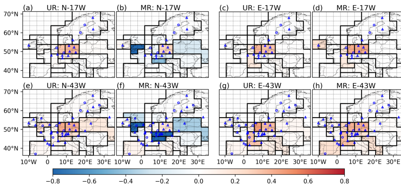
845 Figure 4: Average monthly uncertainty reductions and misfit reductions in FFCO 2 emissions over regions delineated by solid black lines, using the NET17 and NET43 networks and 2-week sampling for the inversions. The first and second columns are the results of INV-N inversions. The third and fourth columns are the results of INV-E inversions. The dashed lines show the grid cells of the transport model LMDZv4. The dots and triangles are the locations of the observation sites where the gradients are extracted with respect to the JFJ reference site. Dots (triangles) correspond to “urban” (or “rural”) stations defined in Sect. 850 2.1. A value of UR and MR closer to unity means a better performance of an inversion to constrain FFCO 2 emissions in a region.
