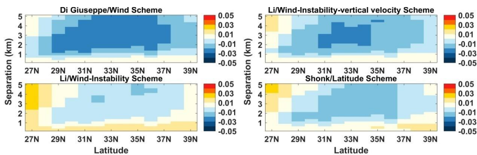
Fig.s1.The zonal difference of cloud cover between calculated and observed for different schemes and its variation with layer separations. The Li/Wind-Instability-vertical velocity
