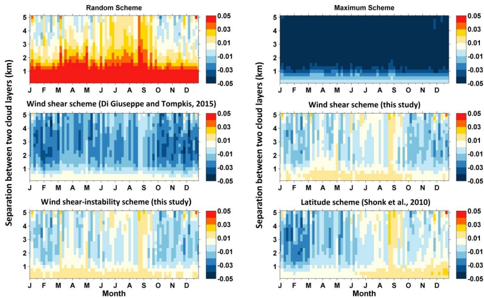
1650 | Figure 6. The monthly differences in cloud cover (unitless) between calculation and observation for different schemes (see the Table 1) and its dependence on the layer separation.
