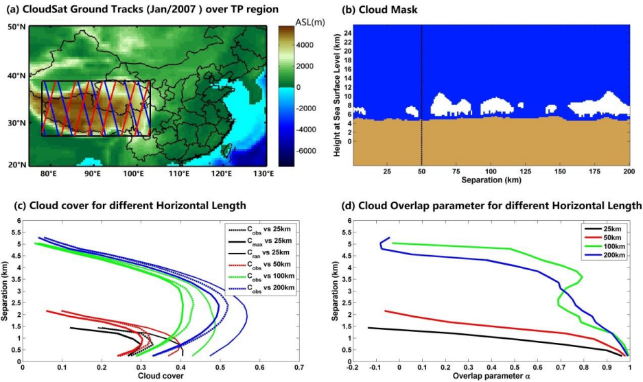
Figure 1. (a) CloudSat overpass tracks (blue line: daytime; red line: nighttime) over the Tibetan Plateau (27 N-39 N; 78 E-103 E); (b) A sample of CloudSat 2B-GEOPROF-LIDAR cloud mask product along the ground track of 200km (white color: cloud fraction>99%; light blue: 0<cloud fraction<99%; deep blue: clear sky; orange color: surface). (c) The observed and calculated segment-average cloud cover profiles based on maximum and random assumptions for different spatial scales and given cloud mask sample in Fig. 1b. (d) The corresponding cloud overlap parameters of contiguous cloud layers for 25, 50, 100 and 200 km spatial scales, respectively. Note that the observations below 1 km over the TP surface have been removed.
