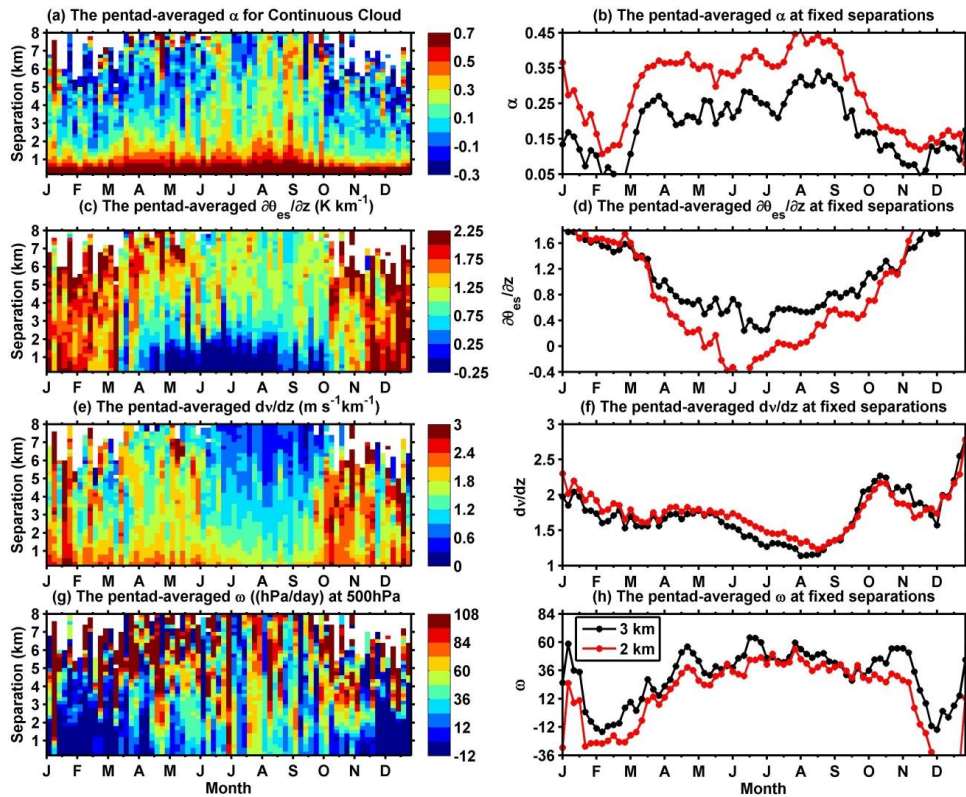
Figure 3. The monthly variations of the pentad-averaged (a) cloud overlap parameter, \alpha , (c) conditional instability to moist convection, \partial\theta_{es}/\partial z ( K km^{-1} ) (e) wind shear, dV/dz ( m s^{-1} km^{-1} ), (g) and vertical velocity \omega (hPa/day) at 500 hPa, for the contiguous cloud layers over the TP ; The monthly variations of the pentad-averaged (b) \alpha , (d) \partial\theta_{es}/\partial z , (f) dV/dz and (h) \omega for the contiguous clouds for the layer separation of 2 km (red) and 3km (black).The monthly variations of the pentad averaged (a) cloud overlap parameter, \alpha , (c) conditional instability to moist convection, \partial\theta_{es}/\partial z , (e) wind shear, dV/dz , (g) and vertical velocity at 500 hPa, \omega for the contiguous cloud layers over the TP ; The monthly variations of the pentad averaged (b) \alpha , (d) \partial\theta_{es}/\partial z , (f) dV/dz and (h) \omega for the contiguous clouds for the layer separation of 2 km (red) and 3km (black).
