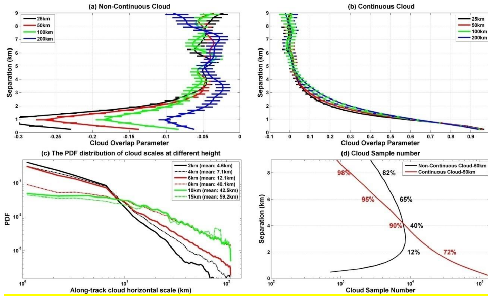
Figure 2. The dependence of \alpha on the layer separation and its sensitivity to the spatial scale for (a) noncontiguous and (b) contiguous cloud pairs; The horizontal bars correspond to means \pm 3 standard error, which represent the upper endpoint and lower endpoint of the 99% confidence interval, respectively, the error bars correspond to \pm 3 standard error; (c) The probability distribution functions (PDFs) of the along-track horizontal scales of cloud system at different height over TP region; (d) The variations of cloud sample number and the cumulative percentages with cloud layer separations for both noncontiguous and contiguous clouds at a given spatial scale of 50km. The cumulative percentages represent the proportions of cloud sample below corresponding layer separation to all samples.
