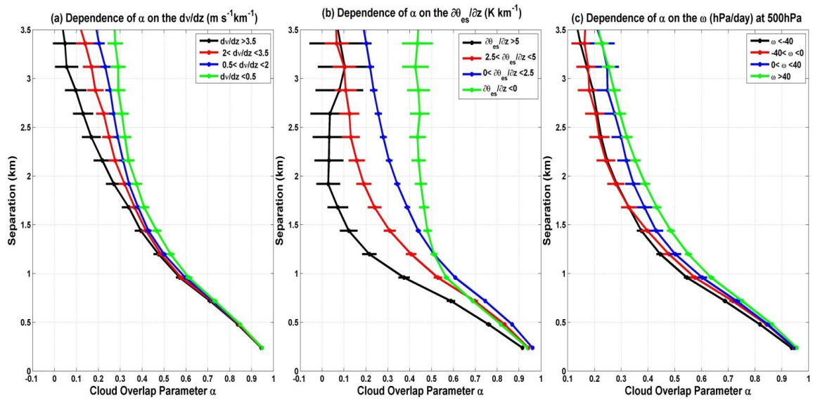
1640 Figure 5. The sensitivities of median overlap parameter \alpha to the (a) wind shear, (b) instability and (c) vertical velocity at 500 hPa at a given upper limit of cloud cover (50%) and spatial scale (50 km) for the contiguous cloud layers. The horizontal bars correspond to means \pm 3 standard error, which represent the upper endpoint and lower endpoint of the 99% confidence interval, respectively. The error bars correspond to \pm 3 1645 standard error.
