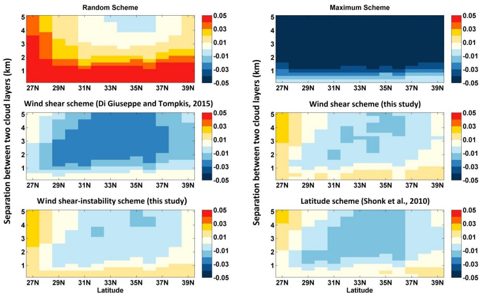
1655 | Figure 7. The zonal differences in cloud cover (unitless) between calculation and observation for different schemes (see the Table 1) and its dependence on the layer separation.
