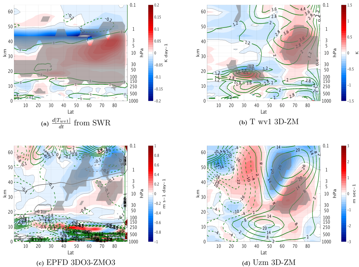
Figure 3. September mean differences between the 3D03 and ZM03 run for all years for temperature wave 1 amplitude tendency from short-wave radiation (3a), temperature zonal wave 1 amplitude (3b), EP flux divergence (3c), and zonal wind (3d) . In Figure 3c the gray line in the upper stratosphere indicates the height where ozone and temperature zonal wave 1 correlation change from positive to negative. Statistically significant areas are shown by gray shading.
