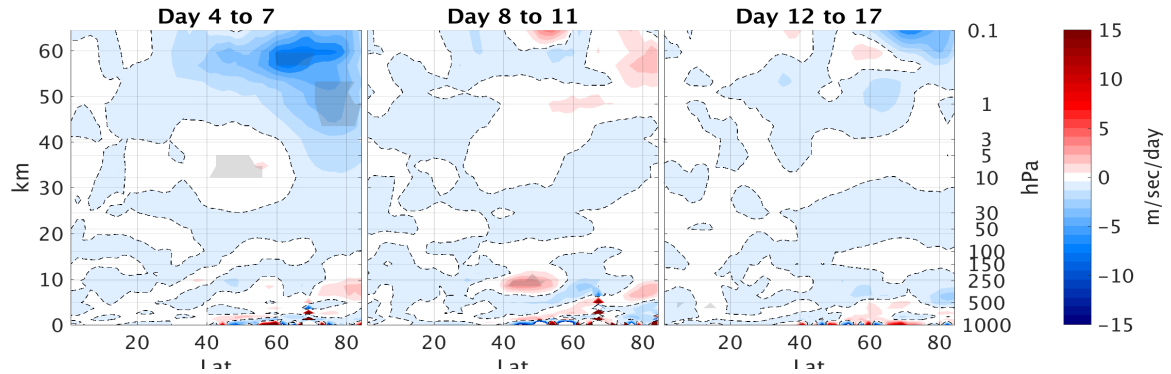
(a) \nabla \cdot F , EQBO, 3D-ZM
