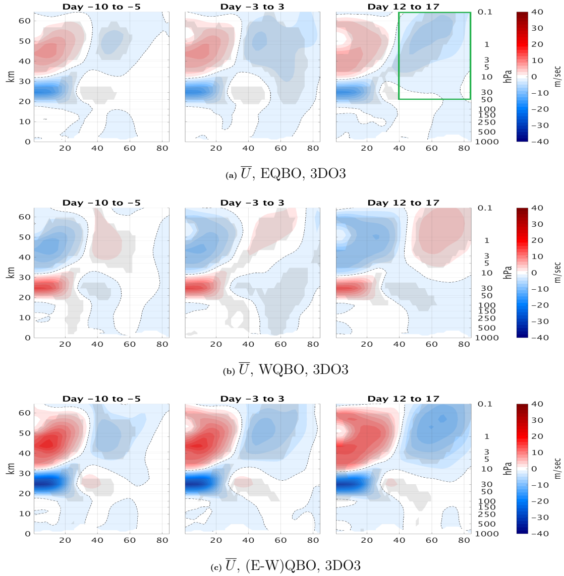
Figure 6. Time lag composite of the zonal mean zonal wind anomalies for east QBO (6a), west QBO (6b), and the difference between them (6c), for the positive heat flux events from the 3DO3 run of October. The green box in Figure 6a shows the area of averaging for Figures 5b-5d.
