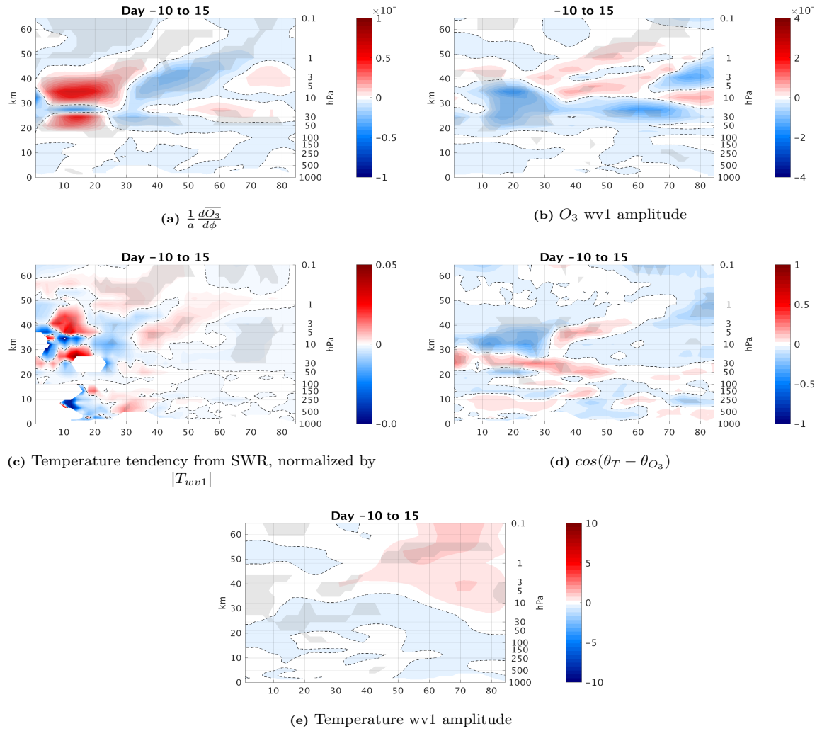
Figure 6. Latitude-height of E-W QBO October positive hat flux events composit for day -10 to 15 (a) Meridional gradient of the zonal mean ozone, (b) wave 1 amplitude of the ozone, (c) temperature wave 1 amplitude tendency from short-wave radiation, (d) ozone-temperature correlation for zonal wave 1, and (e) temperature wave 1 amplitude.
