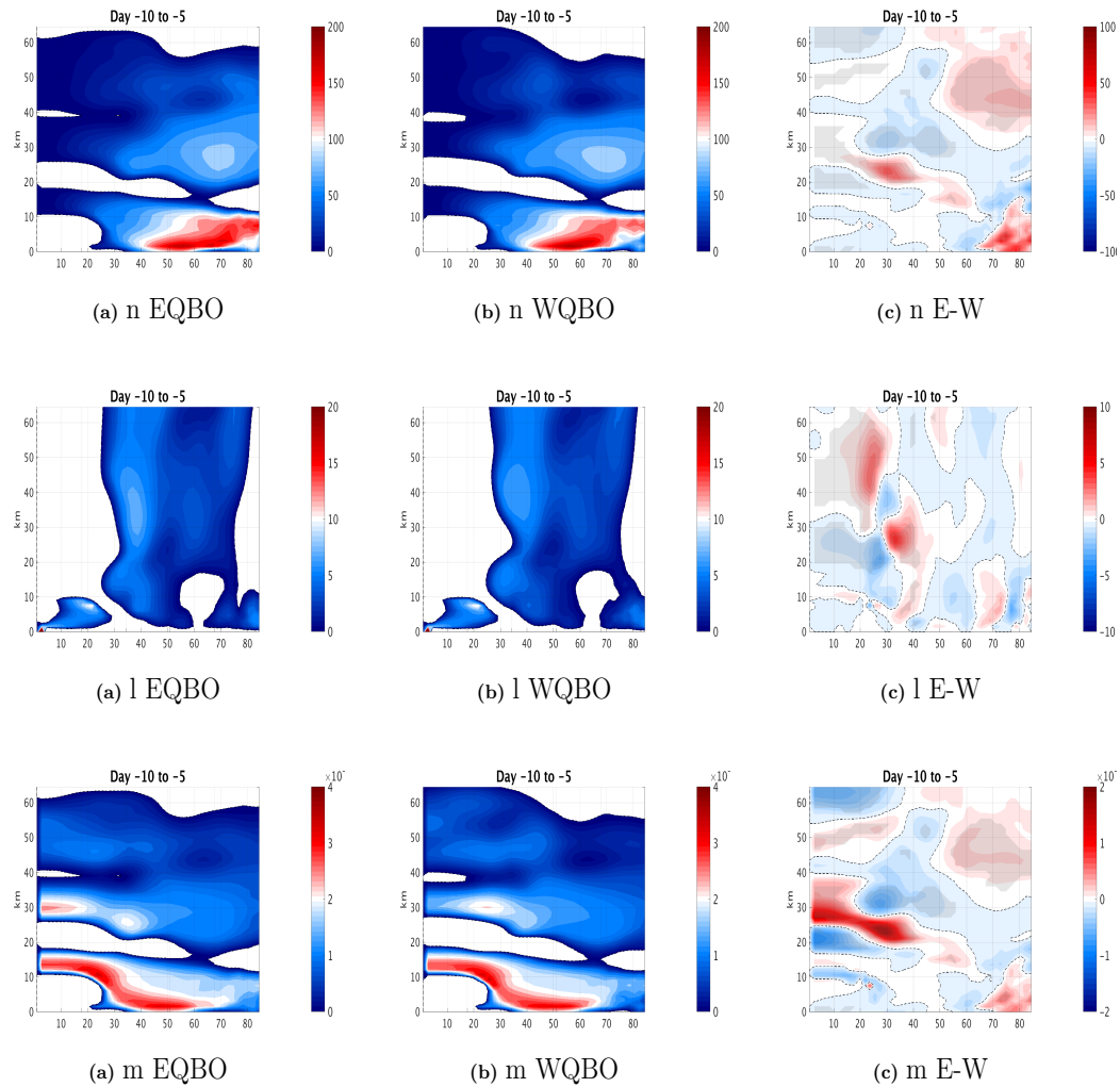
Figure 3. (Top) Index of refraction \left(n^2 = N^2 \left[ \frac{a\bar{q}_y}{\bar{U}-c} - \frac{s^2}{\cos^2\phi} + a^2 f^2 F(N^2) \right] \right) , see eq.C2,5 in Harnik and Lindzen (2001)) at days -10 to -5 for east (left), west (center) and the difference between east and west QBO (right) in the 3DO3 run. The meridional and vertical wave components are shown in the middle and bottom row, correspondingly.
