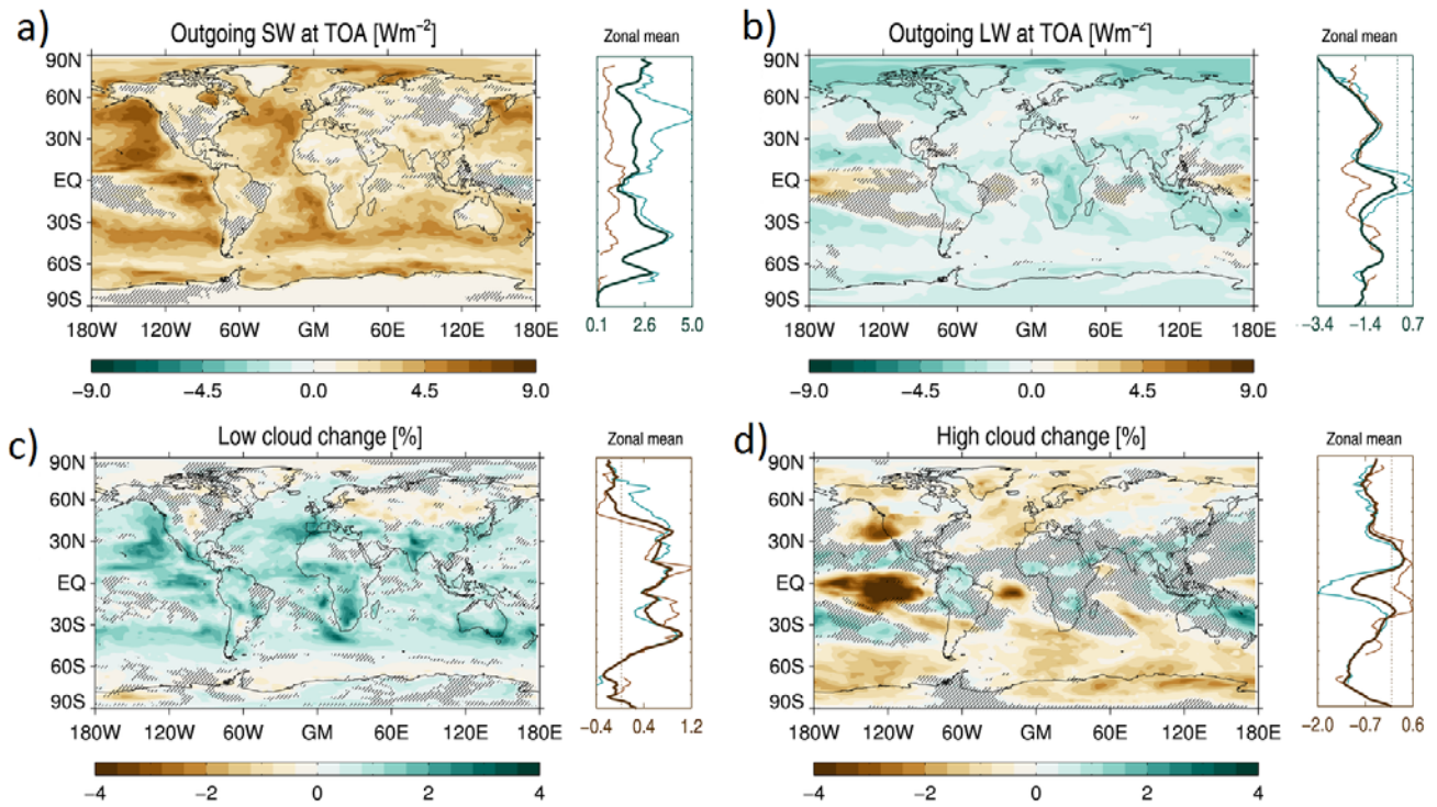
Figure 5: Ensemble median (taken in each grid cell) G4cdnc-RCP4.5 difference of years 2020-2069 of a) outgoing short-wave radiation at TOA ( \text{Wm}^{-2} ), b) outgoing long-wave radiation at TOA ( \text{Wm}^{-2} ), c) change in low cloud fraction (%), and d) change in high cloud fraction (%). Hatched areas are grid cells where less than 75 % of the models agreed on the sign of the change. Zonal averages are given to the right of each panel, where brown and blue lines indicate land-only and ocean-only averages, respectively.
