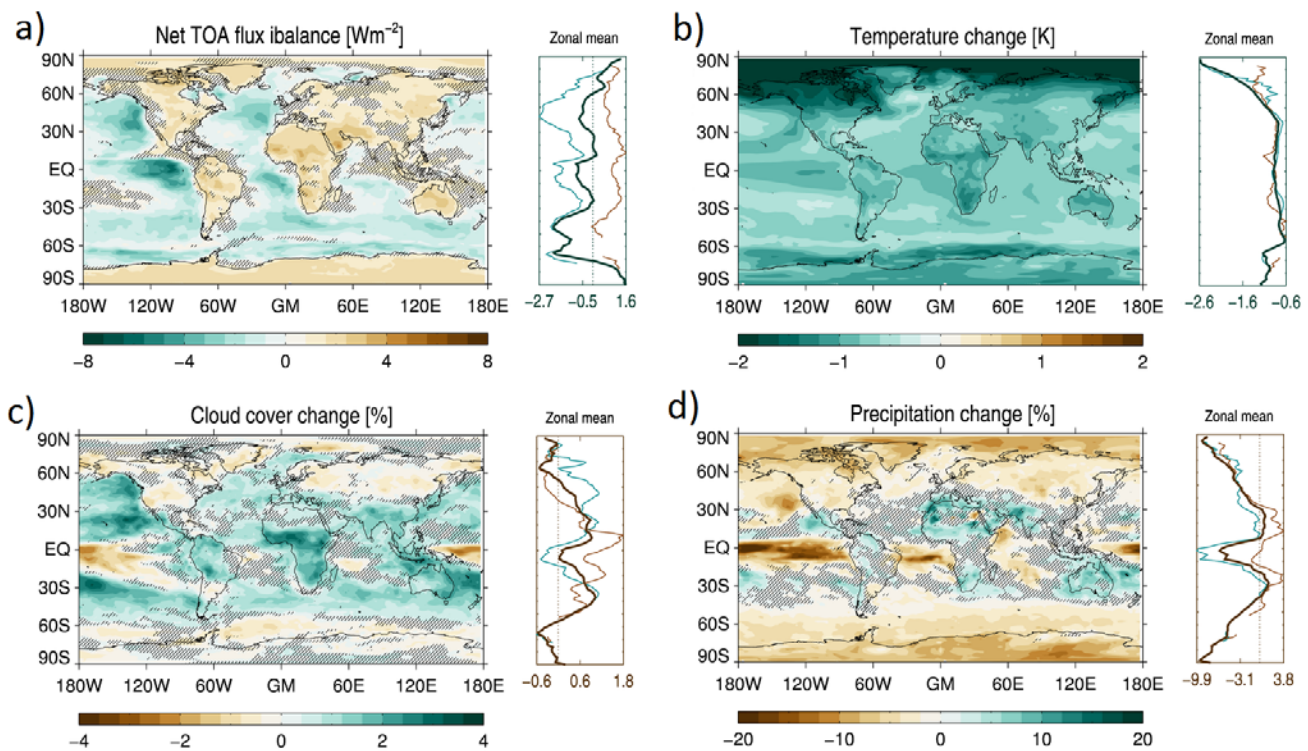
Figure 4: Ensemble median (taken in each grid cell) G4cdnc-RCP4.5 difference based on years 2020-2069 of a) TOA net radiative flux imbalance ( \text{Wm}^{-2} ), b) near-surface air temperature change (K), c) total cloud cover (%), and d) precipitation (%). Hatched areas are grid cells where less than 75 % of the models agreed on the sign of the change. Zonal averages are given to the right of each panel, where brown and blue lines indicate land-only and ocean-only averages. See figures S-2 and S-3 for individual model changes in cloud cover and precipitation, respectively.
