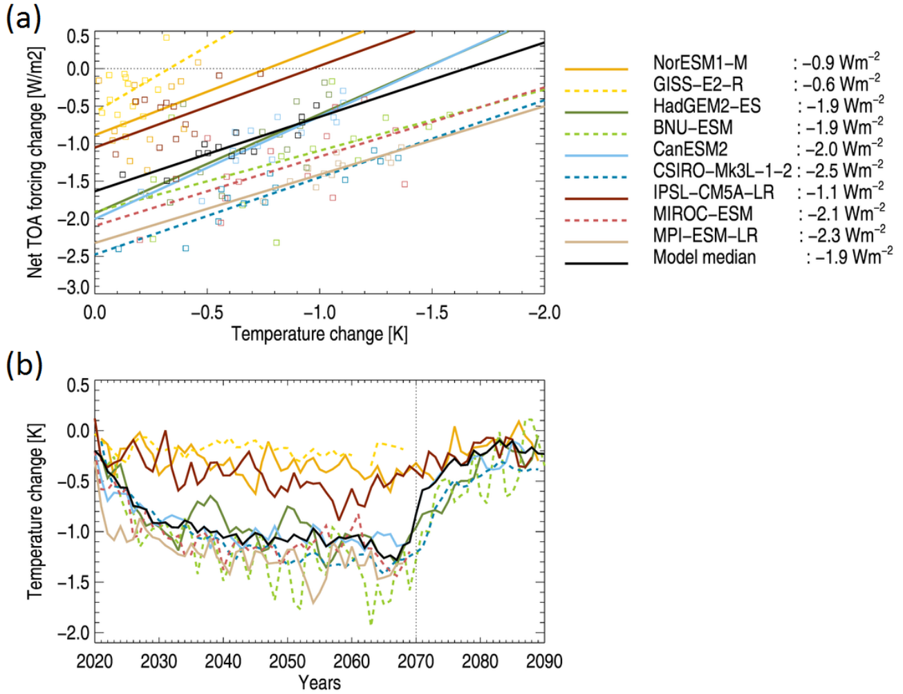
Figure 3: a) Regression of global annual means of the net TOA radiative flux imbalance and near surface temperatures for each model cf. Gregory et al. (2004). Each square represent global annual mean for each of the first ten years and decadal means for the remaining part of the simulations (i.e. last four decades, 2030 - 2069). Numbers to the right gives the intercept – i.e., the effective radiative forcing. b) Time series of the difference in global annual mean near-surface temperature between G4cdnc and RCP4.5 for each model. Dotted vertical line indicates the onset of the termination period.
