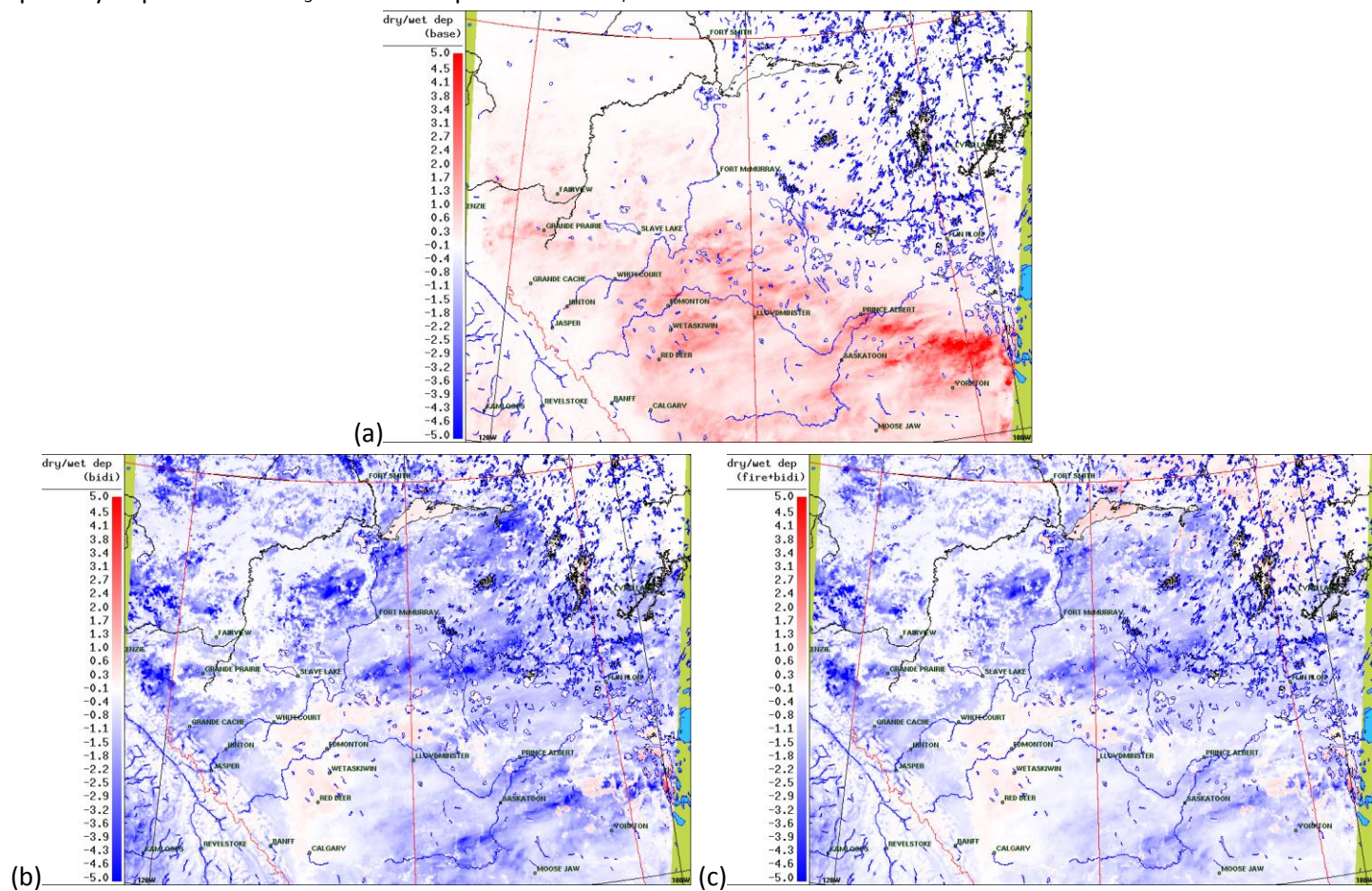
Figure A: Map of dry deposition of \text{NH}_3 over wet deposition of \text{NH}_4^-
