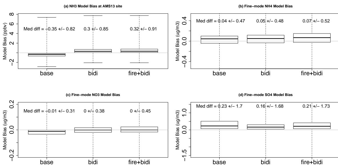
Figure 5. Model-measurement Hourly model-measurement bias in surface (a) \text{NH}_3 , (b) \text{NH}_4^+ , (c) \text{NO}_3^- and (d) \text{SO}_4^{2-} concentrations at the AMS13 ground site in the AOSR.
