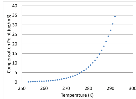
Figure 1. Compensation point ( C_a ) relationship to temperature: C_a for evergreen needleleaf LUC shown as example.
