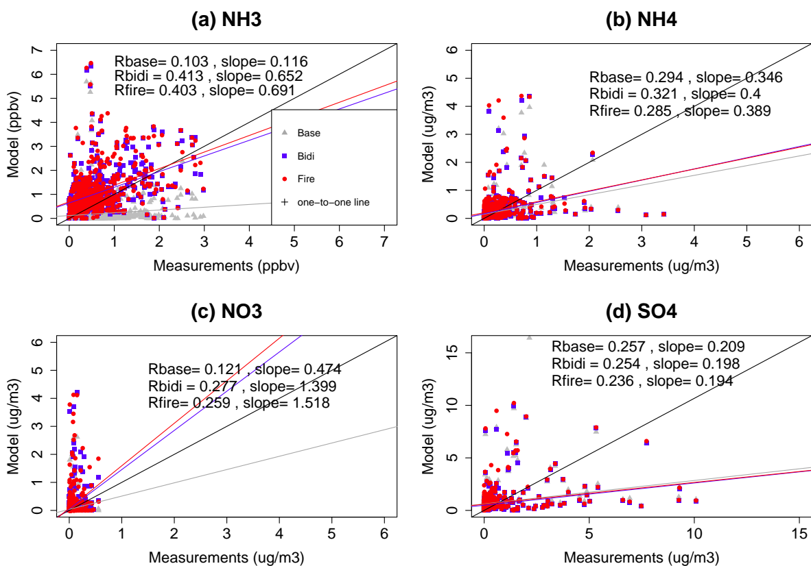
Figure 6. Modelled-Hourly modelled vs measured surface (a) NH 3 , (b) NH 4 + , (c) NO 3 - and (d) SO 4 2- concentrations at the AMS13 ground site in the AOSR. Base model in grey, bidirectional flux model in blue, and fire+bidirectional model in red.
