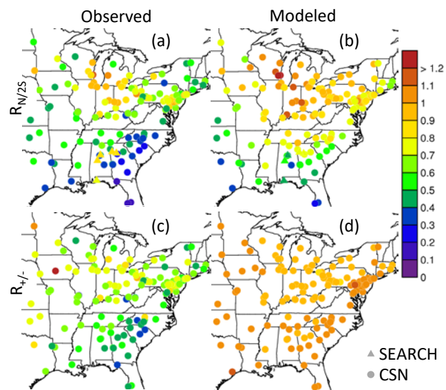
Figure 1. Molar ratio of aerosol ammonium to 2\times sulfate ( R_{N/2S} ) (a-b) and cations to anions ( R_{+/-} ) (c-d) over the eastern US for June 1- July 15, 2013 based on observations and predicted by the CMAQ model.
