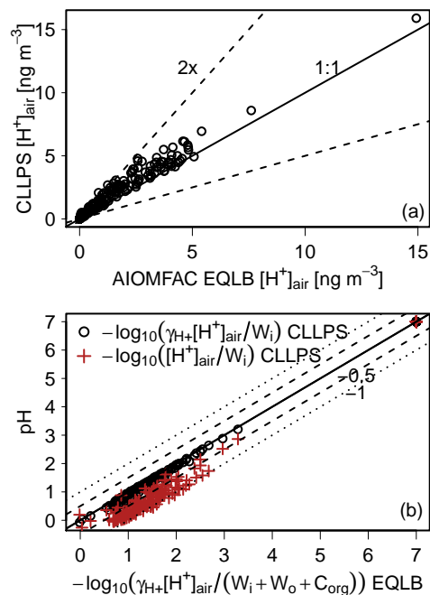
Figure 4. (a) [H + ] air and (b) pH predicted for PM 2.5 using AIOMFAC. Dashed lines in panel (a) indicate a factor of two difference from the 1:1 line. Dashed lines in (b) represent a \pm 0.5 shift in pH while dotted lines represent a \pm 1 shift in pH. Series marked in open circles (○) are summarized in Table 1. All calculations used the ammonium-sodium-sulfate-nitrate-chloride and organic compounds system.
