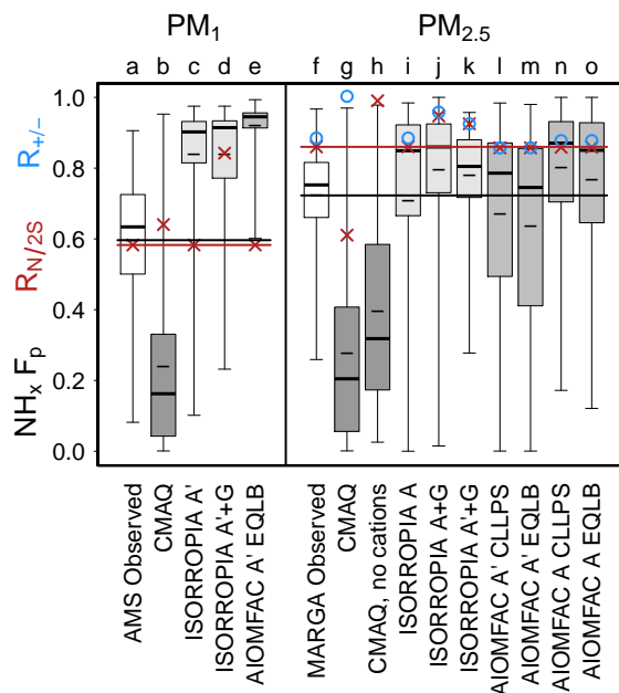
Figure 2. Gas-particle partitioning of ammonia ( \text{NH}_x F_p = \text{ammonium}/(\text{ammonia} + \text{ammonium}) ), mean R_{N/2S} (red \times ), and mean R_{+/-} (blue \circ ) for \text{PM}_{1.0} measured by the Georgia Tech AMS (Xu et al., 2015a) and \text{PM}_{2.5} measured by a MARGA (Allen et al., 2015) as well as predicted by a CMAQ regional chemical transport model calculation and box models for SOAS conditions at CTR. F_p boxplots indicate the maximum, 75th percentile, median, 25th percentile, and minimum. Short dashes within the boxplots indicate the mean F_p . Box model inputs were either the aerosol (A) or aerosol and gas concentrations (A+G). Box models were run with either the ammonium-sulfate system (A') or including all cations and anions (A). AIOMFAC calculations assumed complete liquid-liquid phase separation between the organic-rich and electrolyte-rich phases (CLLPS) or employed a full equilibrium calculation with organic compounds in which phase separation was calculated based on composition (EQLB). Observed gas-phase ammonia concentrations are from the SEARCH network at CTR. Boxplots are labeled by a letter for easier reference in the text. Shading of the boxplot interquartile range distinguishes different models (CMAQ, ISORROPIA, and AIOMFAC). The horizontal lines correspond to mean observed \text{NH}_x F_p (black) and R_{N/2S} (red). A simulation is consistent with observations if it reproduces both \text{NH}_x F_p and R_{N/2S} .
