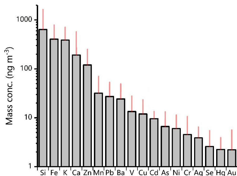
355 Figure 3. Average mass concentrations of 18 trace elements measured in Shanghai as sorted from high to low (log10 scaling). The dark red line indicates one standard deviation.
