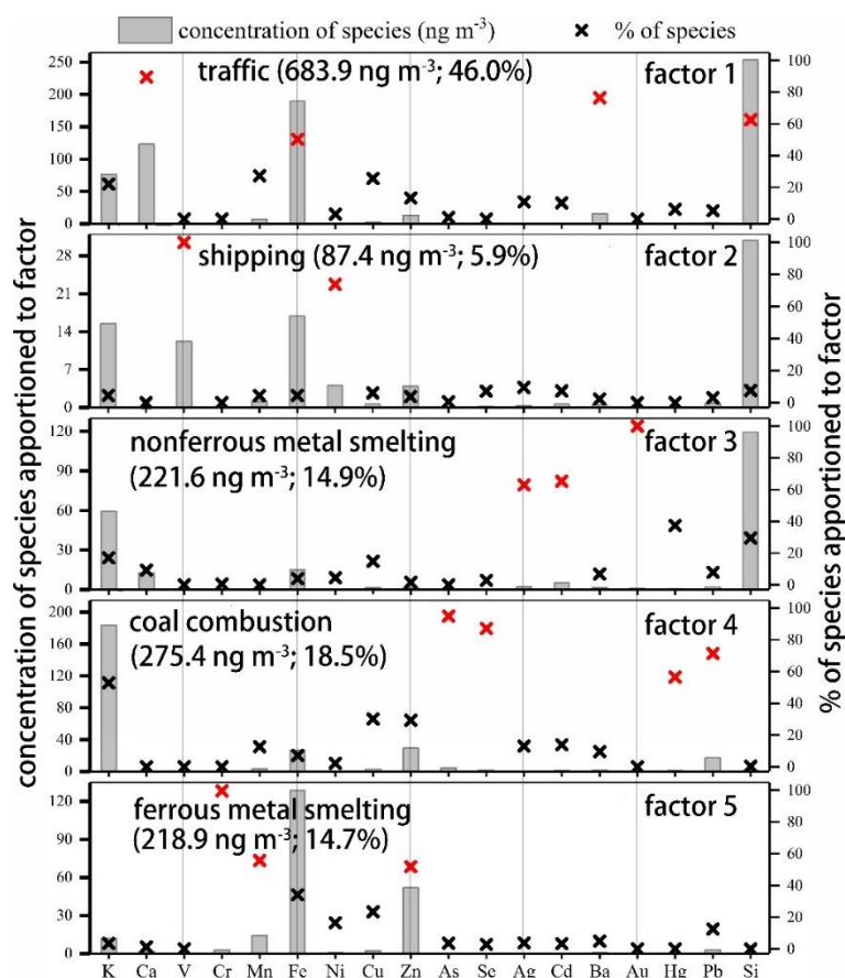
Figure 4. PMF-resolved source profiles (concentration and % of species apportioned
