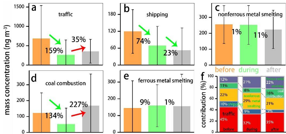
Figure 11. The variation of the overall mass concentration of trace elements contributed by traffic-related (a), shipping (b), nonferrous metal smelting (c), coal combustion (d), and ferrous metal smelting (e), and their relative contributions (f) before, during, and after the total 12 precipitation events.
