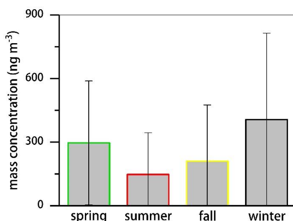
Figure 8. Seasonal variation of elements concentrations contributed by coal combustion in Shanghai. The error bar indicates one standard derivation.
