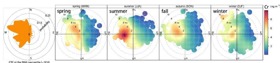
Figure 9. Conditional probability function analysis (left) and bivariate polar plots
