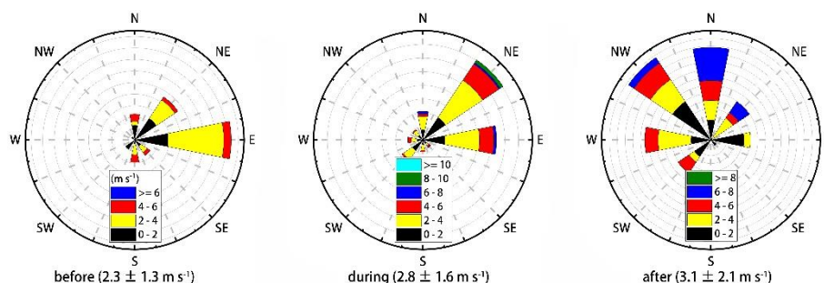
Figure 12. Wind roses plots for the periods before, during, and after the twelve precipitation events. The average wind speed ( \pm 1\sigma ) for each period is shown in bracket.
