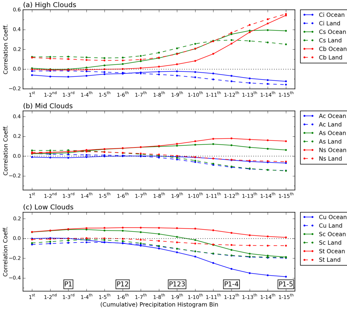
Supplementary Figure 2: Same as Fig. 11, but with the x-axis starting at the 1 st bin and accumulating up to the heaviest 15th bin, which is equivalent to the sum from P1 to P5 or total rainy fraction.
