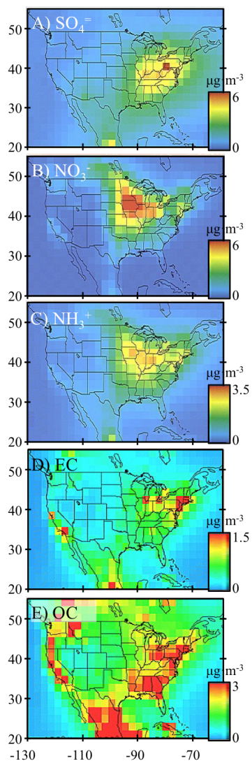
Figure 4. Mean surface concentrations of the (A) \text{SO}_4^{2-} , (B) \text{NO}_3^- , (C) \text{NH}_3^+ , (D) EC and (E) OC in North America obtained in previous studies by GEOS-CHEM modelling validated with the observations in the network IMPROVE (Park et al. 2003, 2004, Copyright by the American Geophysical Union).
