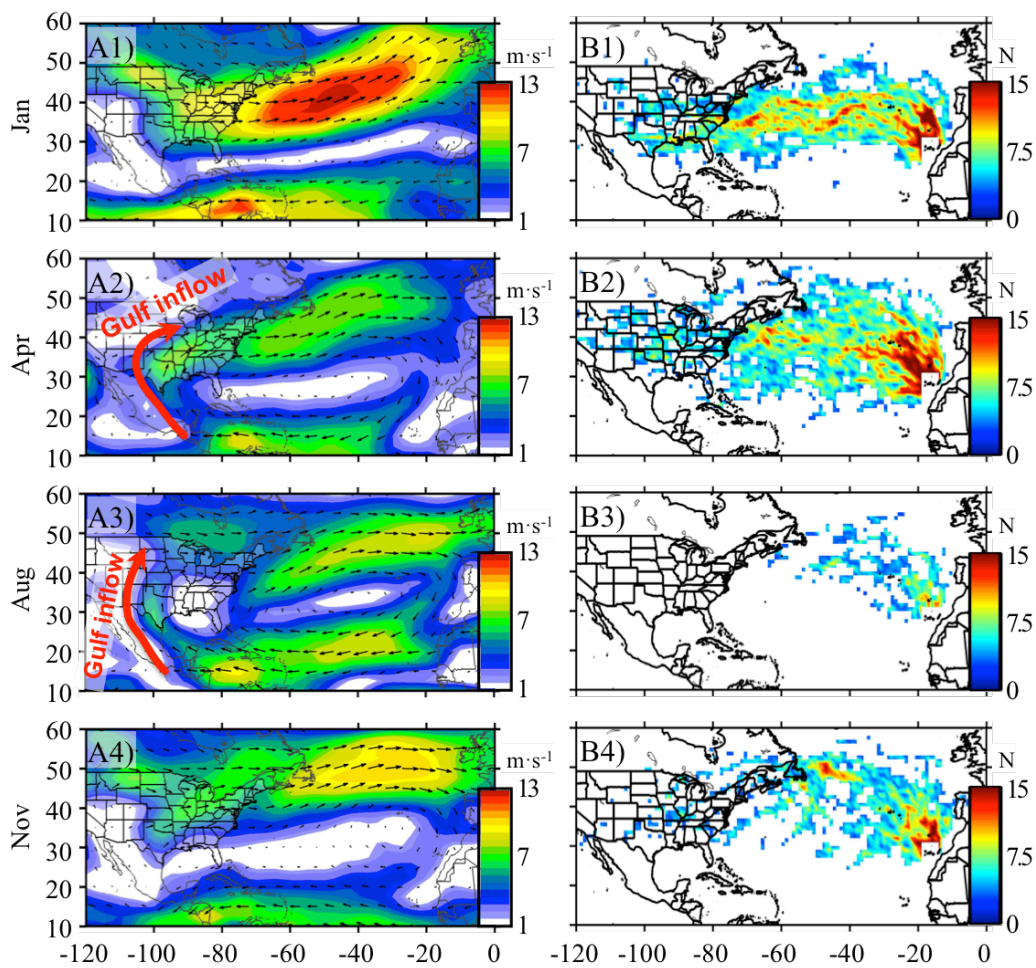
Figure 2. (A) Wind vector at 850 mb and (B) Transport Route Frequency (TRF) for January (Jan), April (Apr), August (Aug) and November (Nov) of the period 2008–2013. The Gulf inflow is highlighted.
