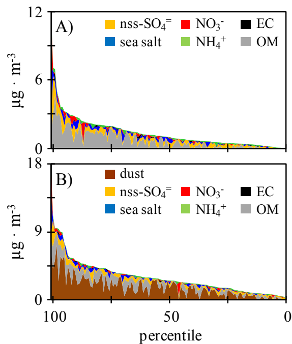
Figure 10. Contribution of each aerosol specie to bulk PM 10 in samples collected at Izaña under westerly airflow conditions; data classified from the highest to the lowest levels. (A) Considering mayor components except dust. (B) Considering all mayor components including mineral dust.
