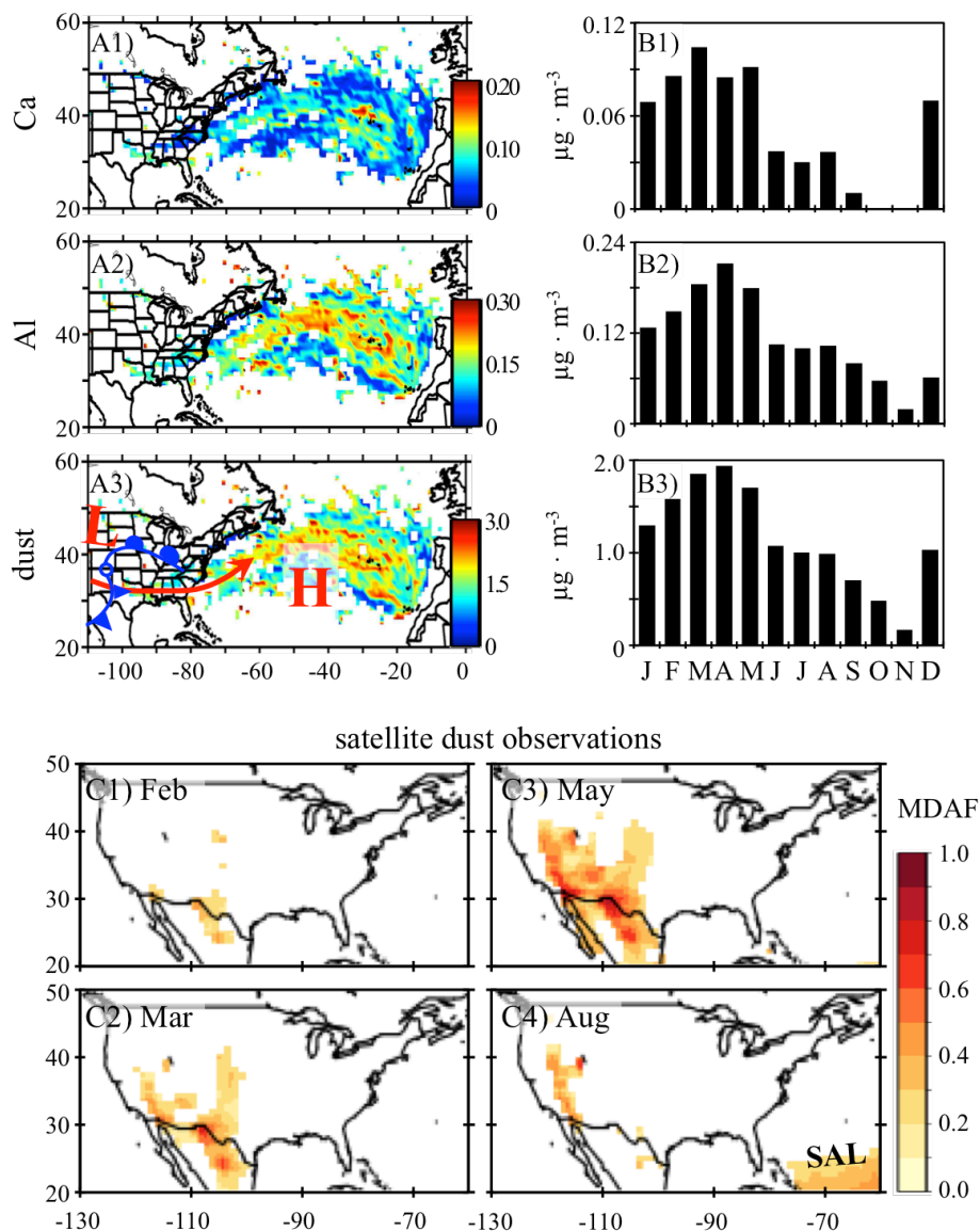
Figure 8. (A) Median Concentration At Receptor (MCAR) plots and (B) monthly median distribution for calcium (Ca), aluminium (Al) and dust, and (C) Mean 2008-2013 Aerosol index averaged (data source: http://disc.sci.gsfc.nasa.gov/ ). The MCAR plots maximum concentration tick label includes concentration higher than this upper limit.
