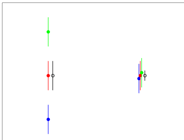
Figure 12. Colored error bars: individual anomalies, black: merged (median) anomaly.
