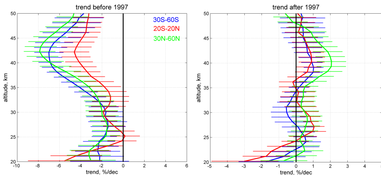
5 Figure 11. Vertical profiles of ozone trends obtained by the multiple regression Eq.(9), in 1984-1997 (left) and in 1998-2016 (right), for broad latitude bands. Error bars are 2\sigma uncertainties.
