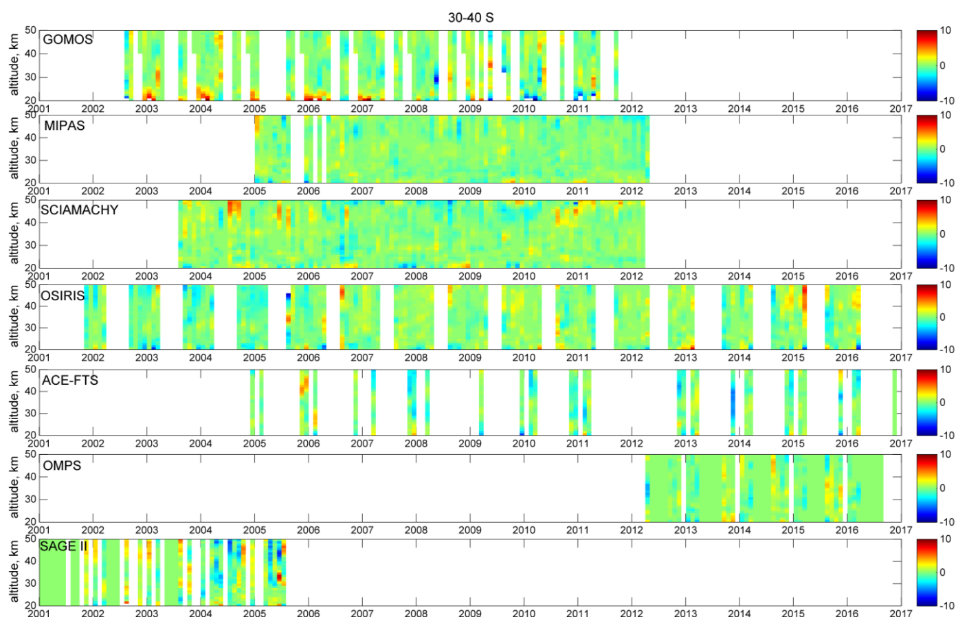
10 Figure 5. Deviations (in %, color) of deseasonalized anomalies for GOMOS, MIPAS, SCIAMACHY, OSIRIS, ACE-FTS, OMPS and SAGE II (indicated in the panels) from the median deseasonalized anomalies computed using all datasets, \Delta_k - \Delta_{median} . Latitude band is 30-40°S.
