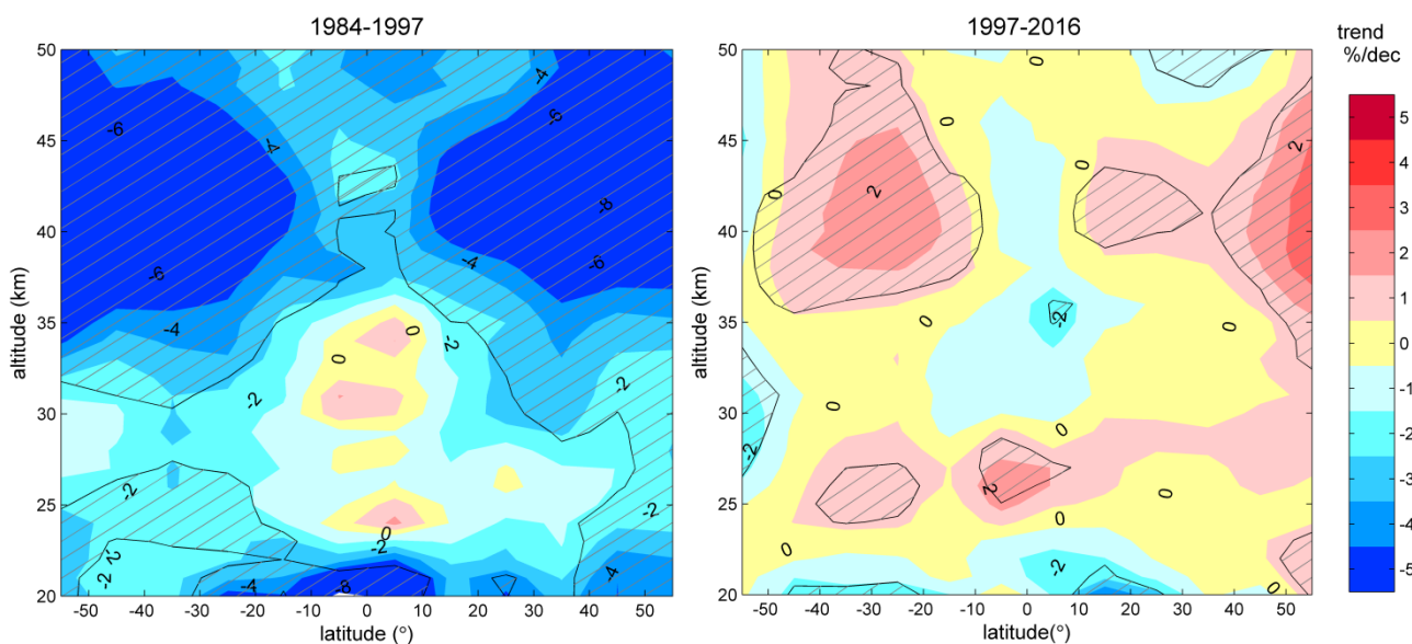
Figure 10. The ozone trend in % per decade for different latitudes for 1984–1997 (left) and 1997–2016 (right). Shaded areas show regions where trends are statistically different from zero at the 95% level.
