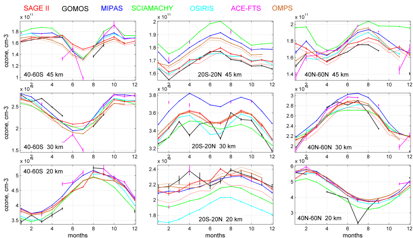
5 Figure 3. Ozone seasonal cycle for latitudes 40°-60°S (left), 20°S-20°N (center) and 40°-60°N (right), for altitudes 45 km (top row), 30 km (center row) and 20 km (bottom row). Error bars are 2 \sigma uncertainties according to Eq.(5). Dashed lines indicate corrected seasonal cycle for SAGE II and OMPS, see text for explanation. The seasonal cycles in the indicated zones are computed as the mean of seasonal cycles in 10° latitude bands.
