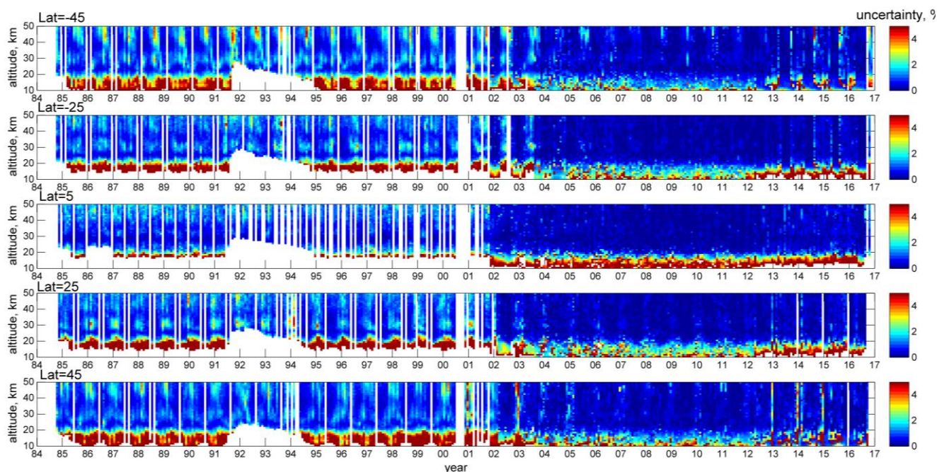
5 Figure 9. Uncertainties of the merged deseasonalized anomalies in %, Eq.(8), for several 10° latitude bands, centers of which are specified in the legend.
