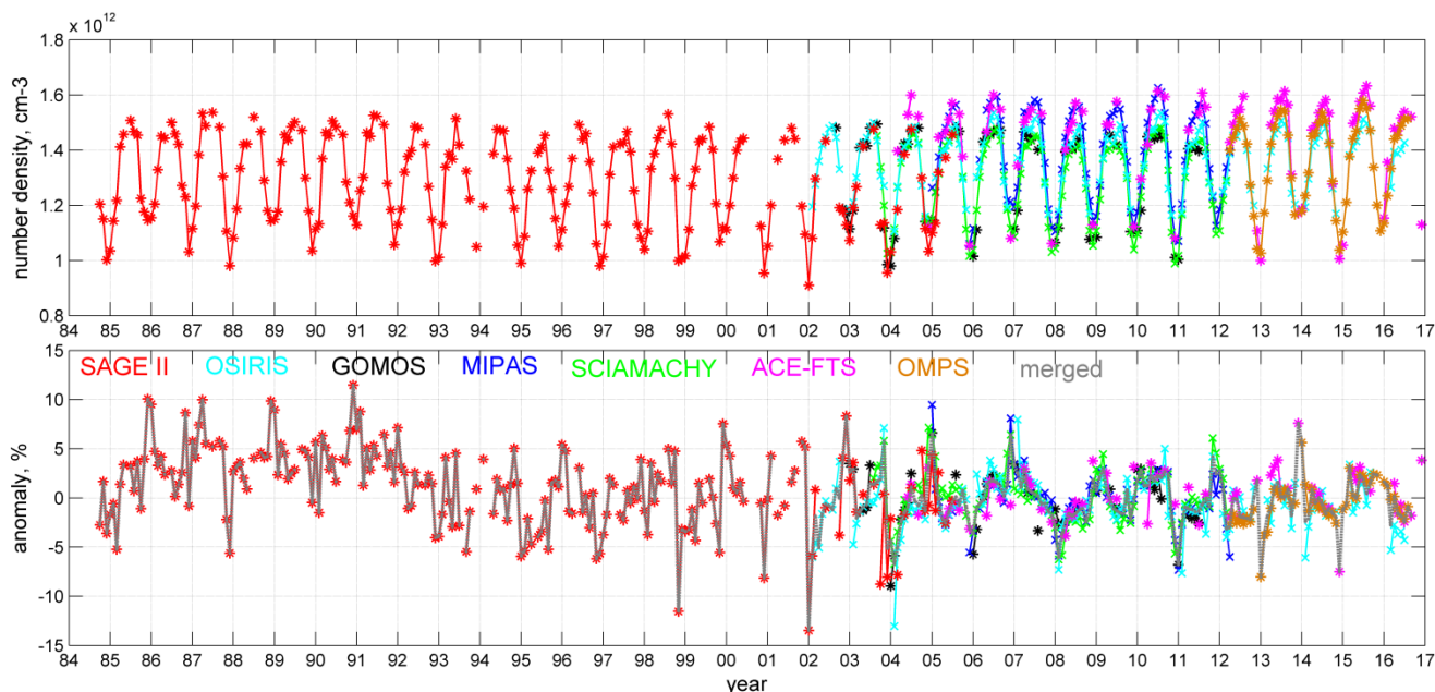
Figure 6. Top: monthly zonal mean ozone at 35 km in the latitude band 40°-50°N. Bottom: individual deseasonalized anomalies and the merged anomaly (grey dashed line).
