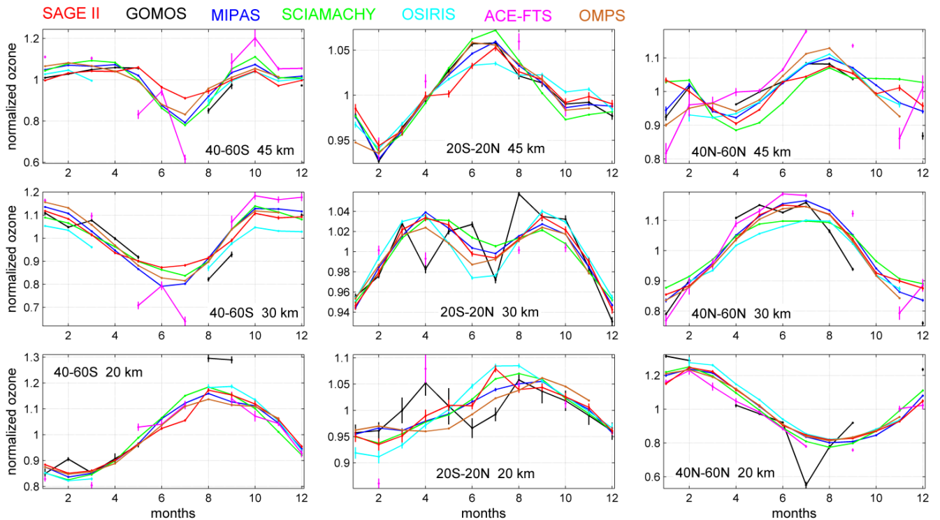
Figure 4. Ozone seasonal cycle normalized on the mean ozone value for latitudes 40-60S (left), 20S-20N (center) and 40-60 N (right), for altitudes 45 km (top row), 30 km (center row) and 20 km (bottom row). Error bars are 2\sigma uncertainties according to Eq.(5).
