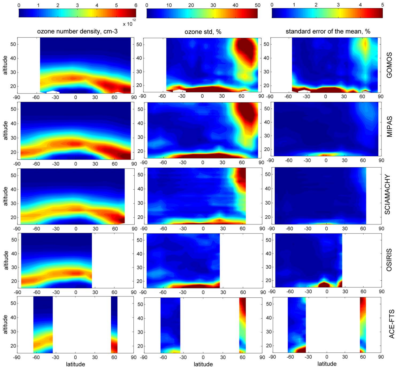
5 Figure 2. Left: monthly zonal mean ozone profiles for January 2008 for Ozone_cci instruments, center: sample variability in %, right: standard error of the mean calculated using Eq. (2).
