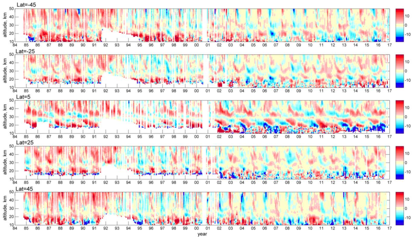
5 Figure 8 Examples of merged deseasonalized anomalies (color: %), for several 10° latitude bands, centers of which are specified in the legend.
