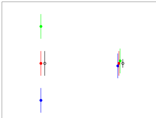
Figure 12. Schematic illustration (arbitrary y-axis scaling) of two extreme cases of individual anomalies and their uncertainties. Colored error bars: individual anomalies, black: merged (median) anomaly. Left: significantly different individual anomalies with non-intersecting error bars, right: nearly coinciding individual anomalies.
