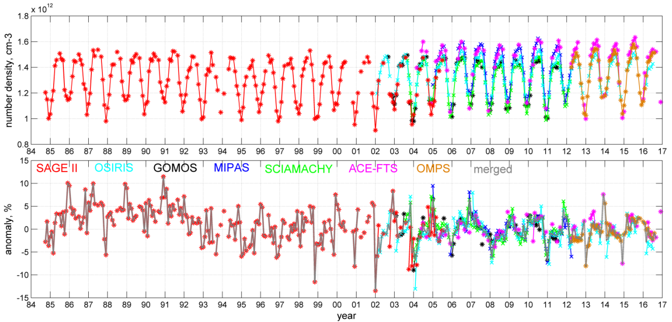
10 Figure 6. Top: monthly zonal mean ozone at 35 km in the latitude band 40°-50°N. Bottom: individual deseasonalized anomalies and the merged anomaly (grey line).
