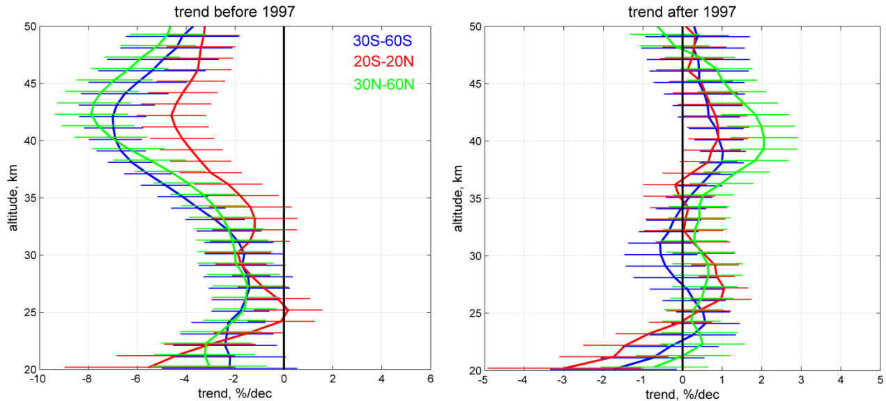
5 Figure 11. Vertical profiles of ozone trends obtained by the multiple regression Eq.(9), in 1984-1997 (left) and in 1998-2016 (right), for broad latitude bands. Error bars are 2\sigma uncertainties.
