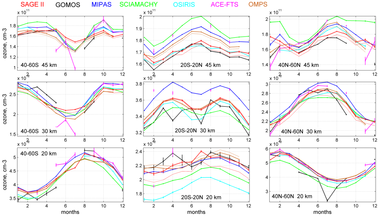
Figure 3. Ozone seasonal cycle for latitudes 40°-60°S (left), 20°S-20°N (center) and 40°-60°N (right), for altitudes 45 km (top row), 30 km (center row) and 20 km (bottom row). Error bars are 2\sigma uncertainties according to Eq.(5). Dashed lines indicate corrected seasonal cycle for SAGE II and OMPS, see text for explanation. The seasonal cycles in the indicated zones are computed as the mean of seasonal cycles in 10^\circ latitude bands.
