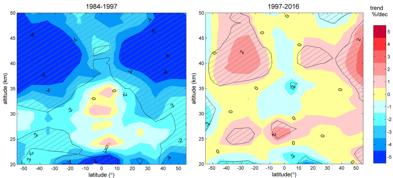
10 Figure 10. The ozone trend in % per decade for different latitudes for 1984–1997 (left) and 1997–2016 (right). Shaded areas show regions where trends are statistically different from zero at the 95% level.
