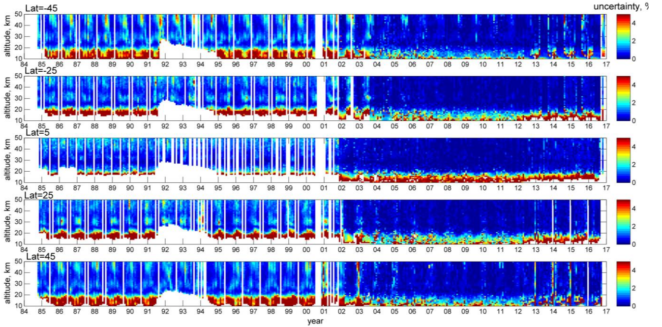
5 Figure 9. Uncertainties of the merged deseasonalized anomalies in %, Eq.(8), for several 10^\circ latitude bands, centers of which are specified in the legend.
