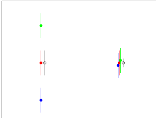
15 Figure 12. Schematic illustration (arbitrary y-axis scaling) of two extreme cases of individual anomalies and their uncertainties. Colored error bars: individual anomalies, black: merged (median) anomaly. Left: significantly different individual anomalies with non-intersecting error bars, right: nearly coinciding individual anomalies.
