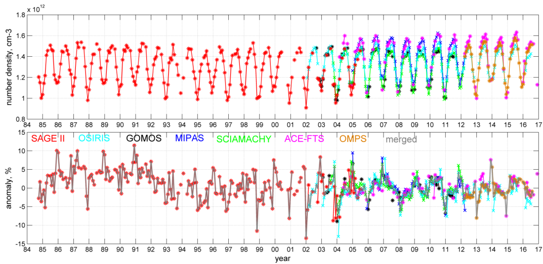
10 Figure 6. Top: monthly zonal mean ozone at 35 km in the latitude band 40°-50°N. Bottom: individual deseasonalized anomalies and the merged anomaly (grey line).
