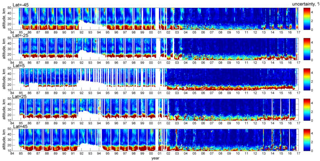
Figure 9. Uncertainties of the merged deseasonalized anomalies in %, Eq.(8), for several 10° latitude bands, centers of which are specified in the legend.
